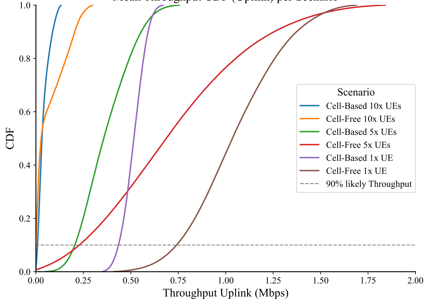
Mean Throughput CDF (Uplink) per Scenario
