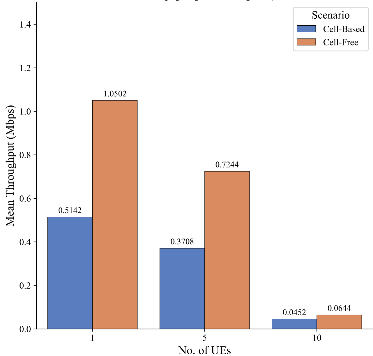
Throughput per UE (Uplink)
