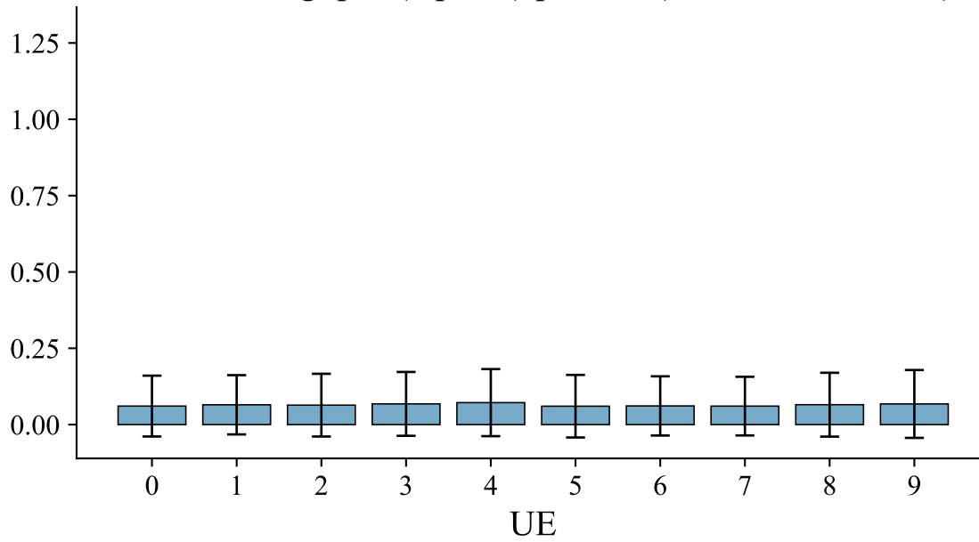
Mean Throughput (Uplink) per UE (Cell-Free, 10 UEs)
