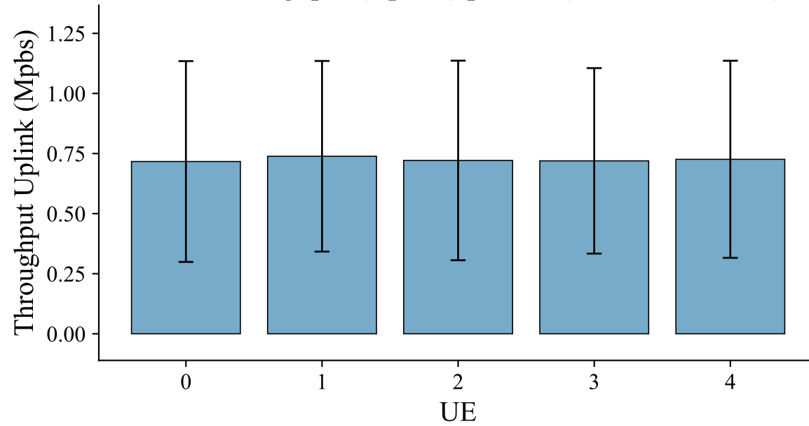
Mean Throughput (Uplink) per UE (Cell-Free, 5 UEs)
