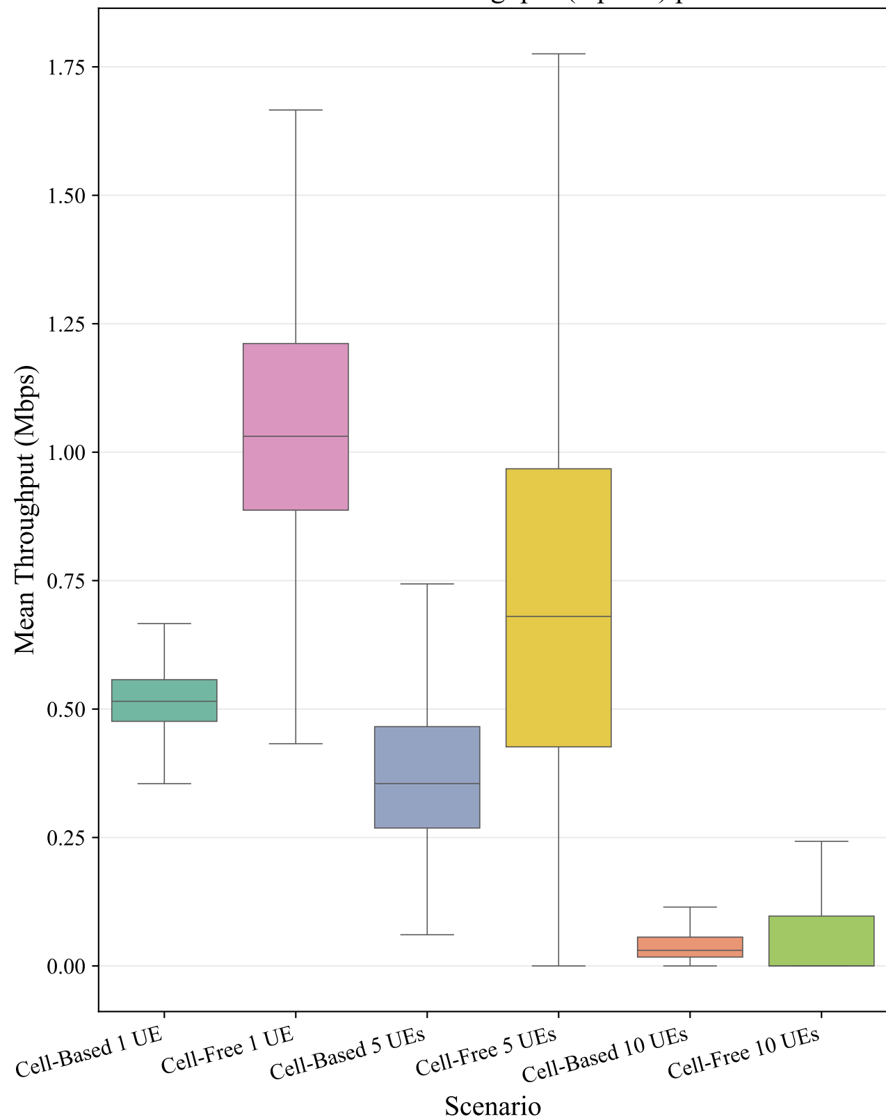
Distribution of Mean Throughput (Uplink) per Scenario
