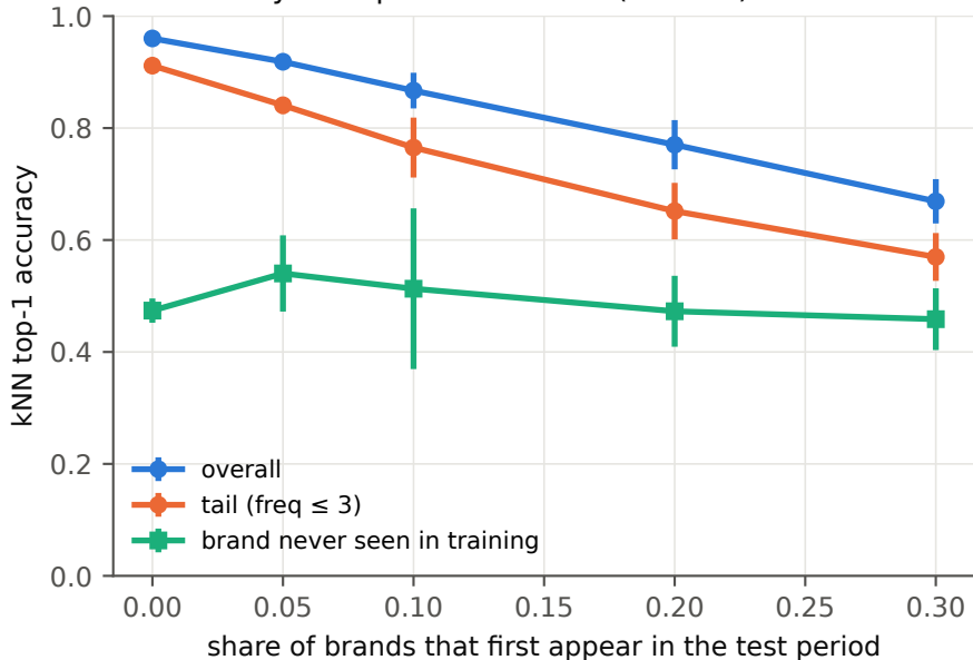
Tail severity sweep: novel brands ( \alpha = 1.1 )
