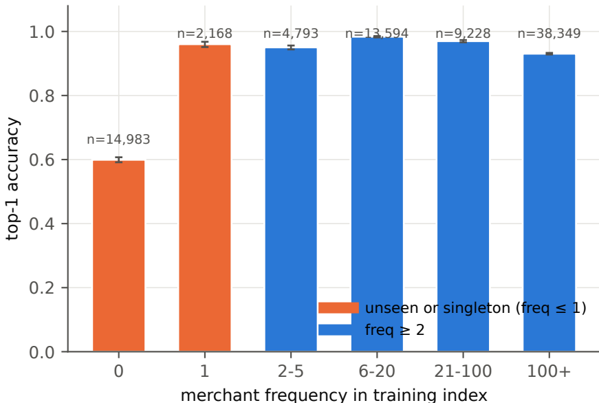
kNN top-1 accuracy by training frequency
