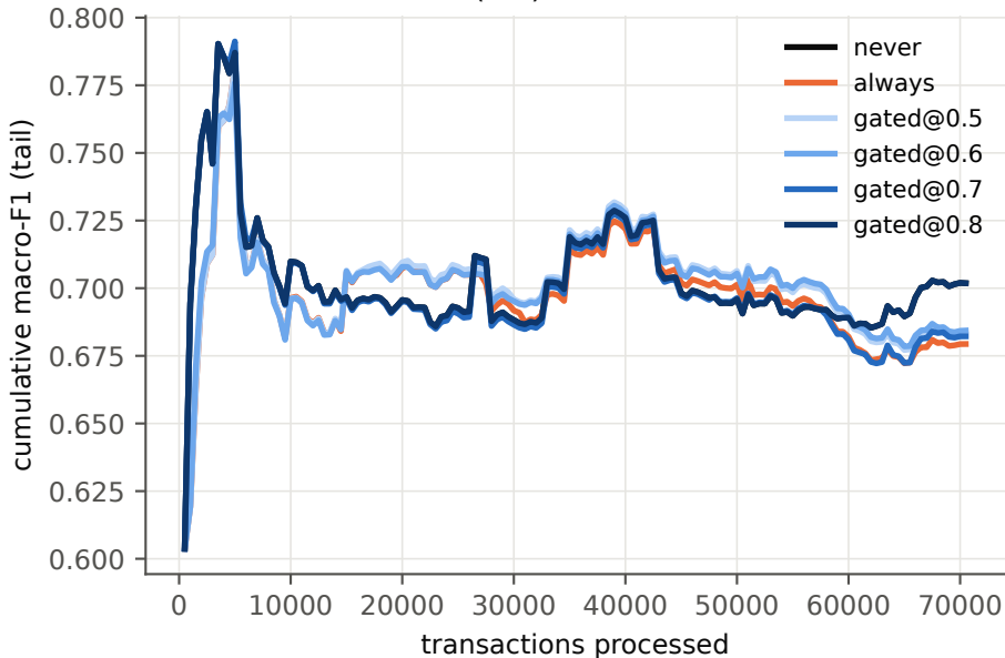
Cumulative macro-F1 (tail)
