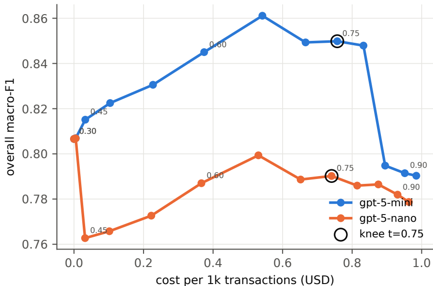
Accuracy-cost frontier over the gate threshold
