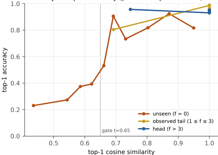
Accuracy vs top-1 similarity (per-series quantile bins)
