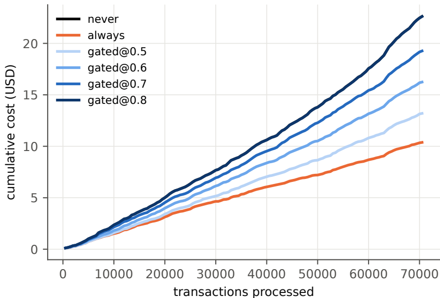
Cumulative fallback cost
