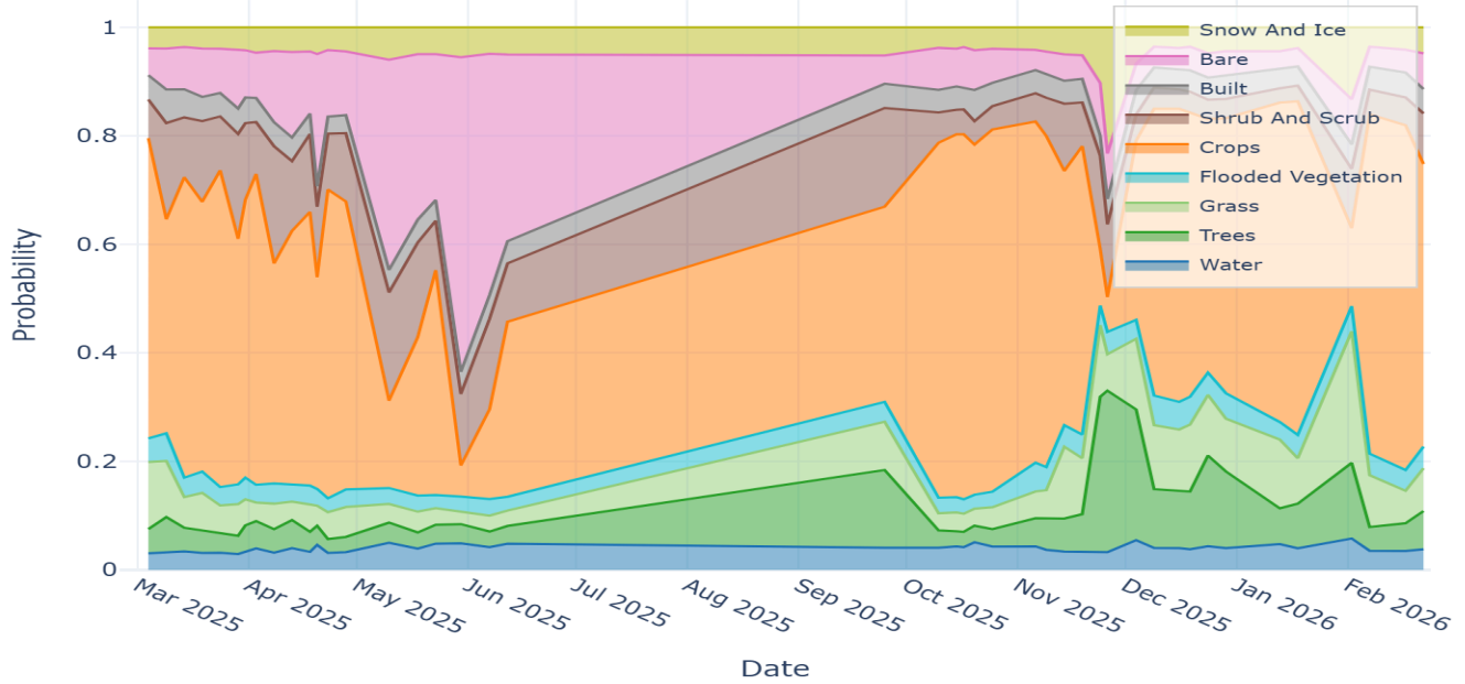
Land Class Probabilities (Dynamic World)
