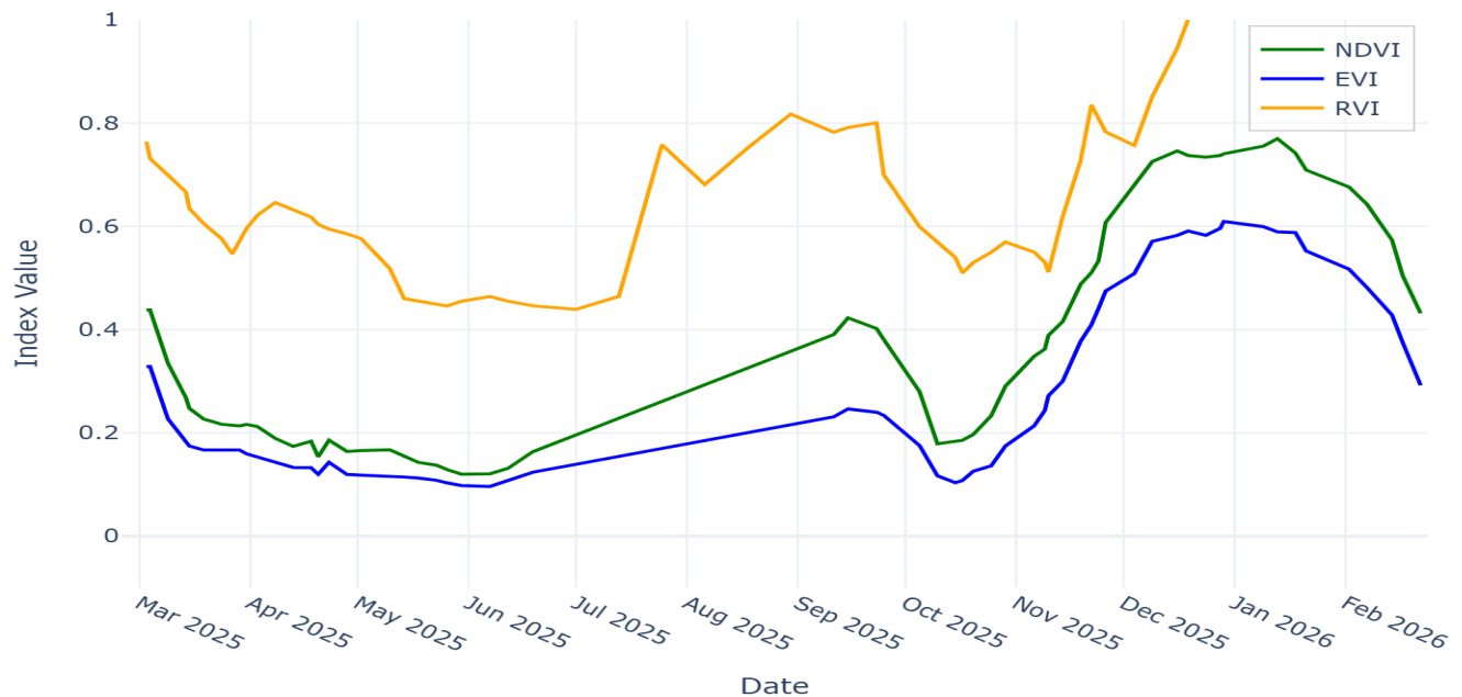
Vegetation Indices (NDVI, EVI, RVI)
