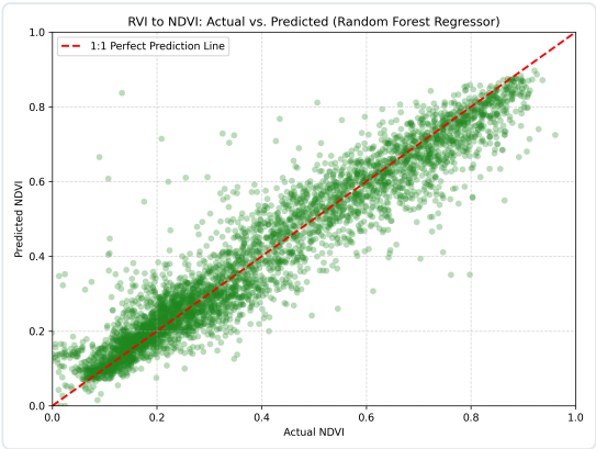
Figure 5: Predicted vs Ground-truth NDVI (Test Split)
