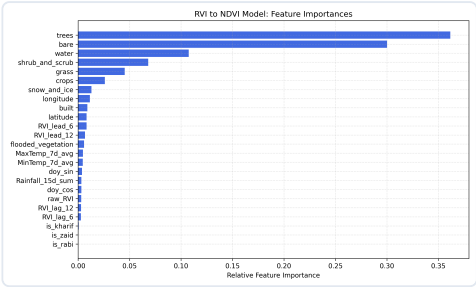
Figure 6: Model Relative Feature Importances
