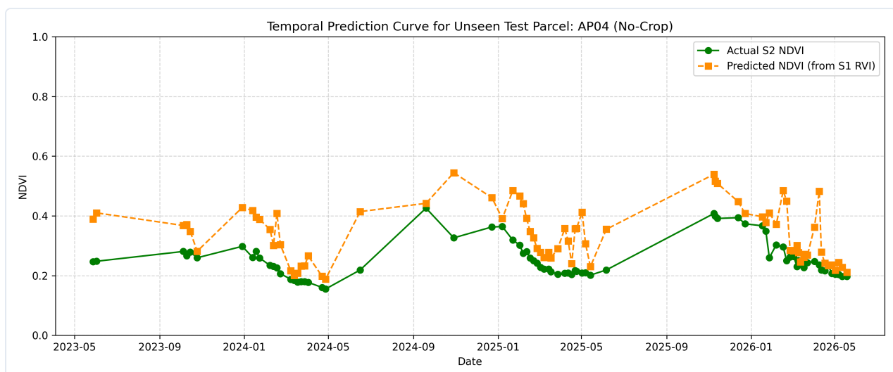
Figure 3: Synthetic NDVI curve predictions vs actual Sentinel-2 optical NDVI on an unseen test parcel.
