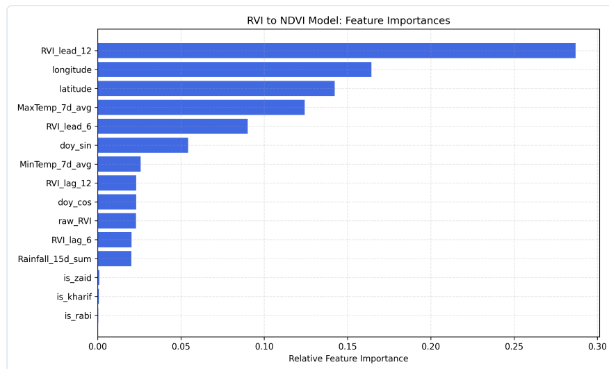
Figure 2: Relative feature importances in Random Forest regressor.
