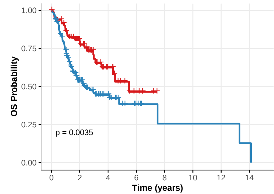
BRCA1
