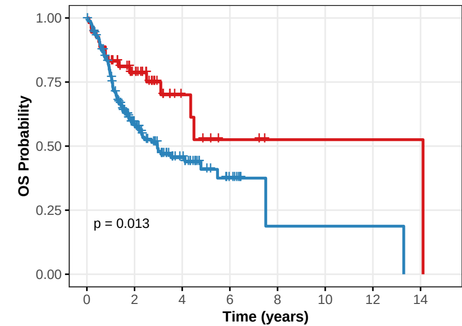
H2AX
