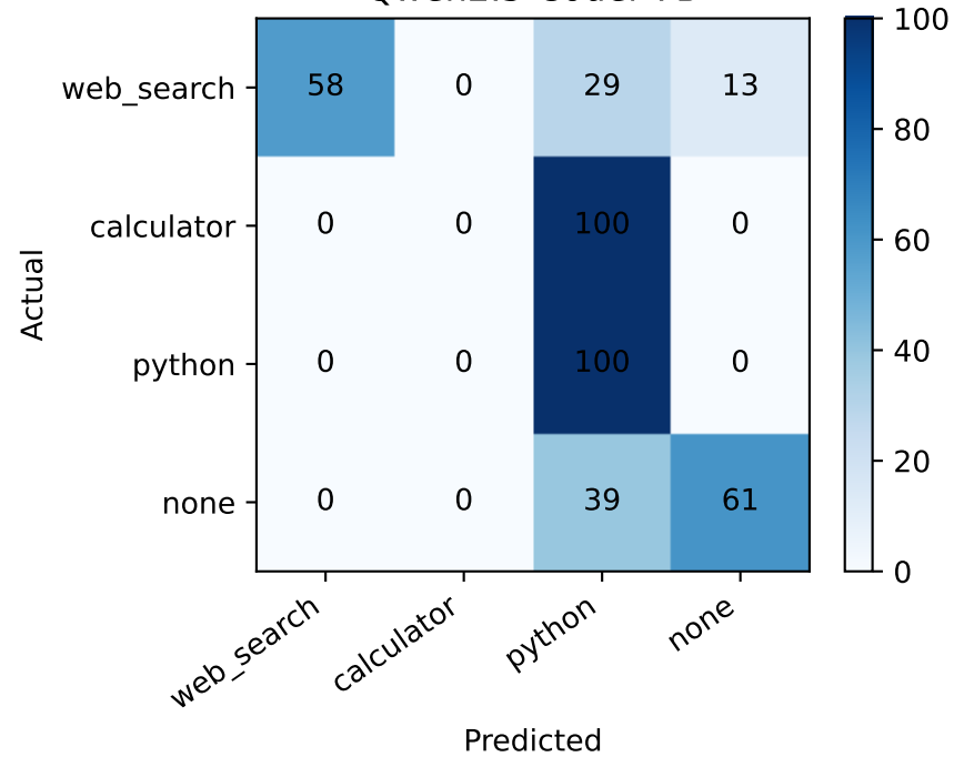
Qwen2.5-Coder-7B
