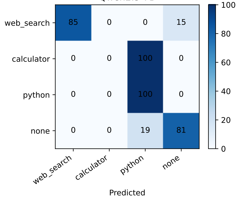
Qwen2.5-7B
