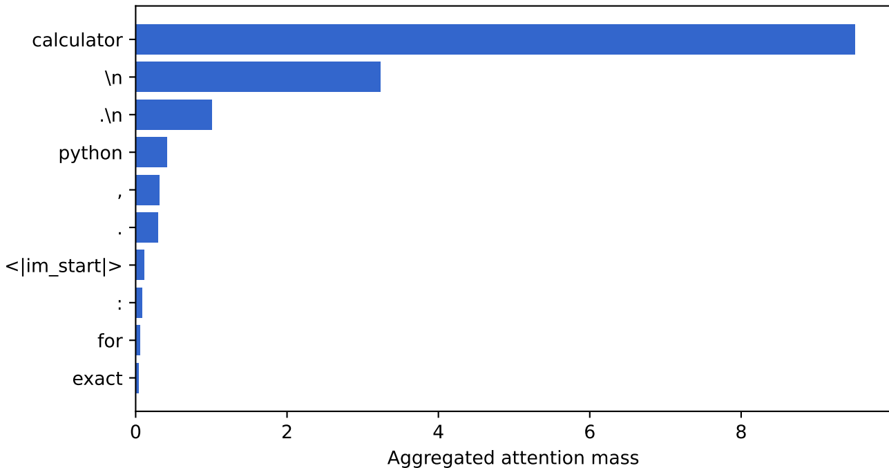
L26H4 attention on calculator prompts
