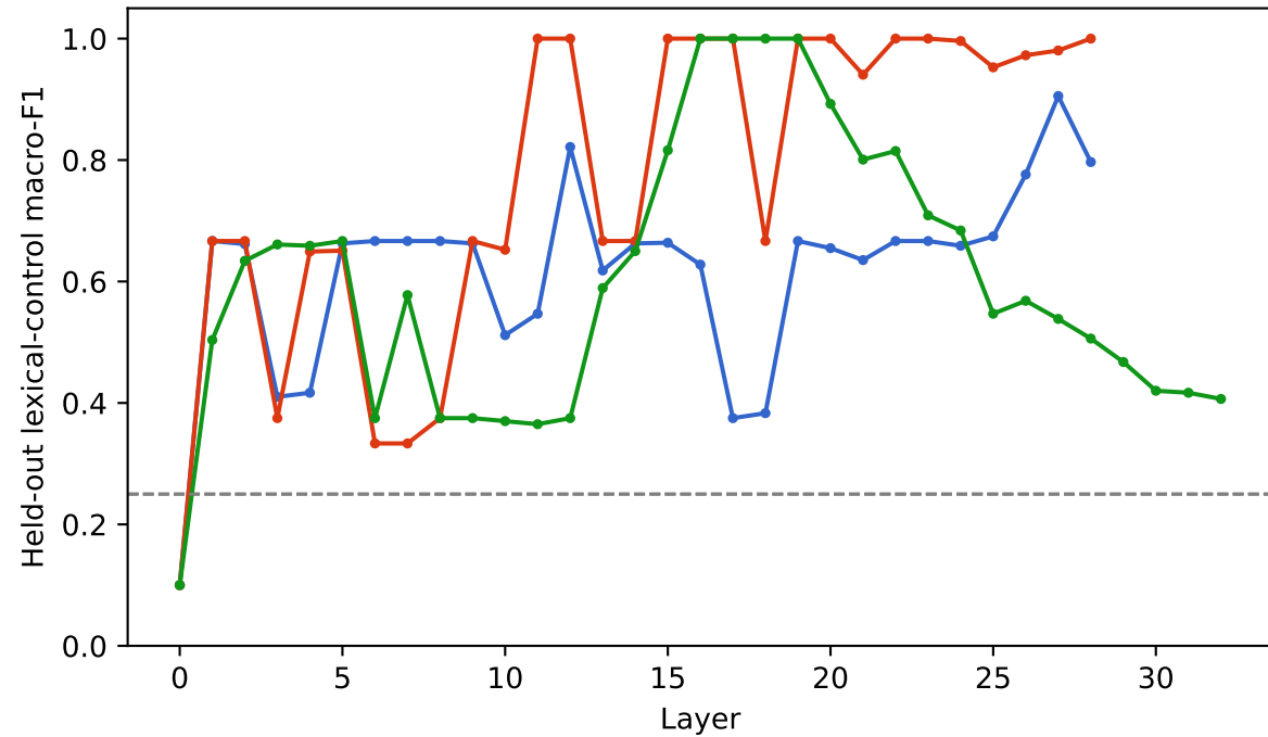
Residual stream
