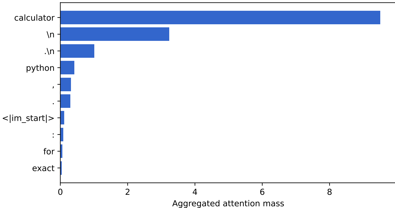
L26H4 attention on calculator prompts
