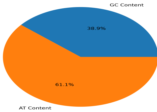
GC vs AT Content
