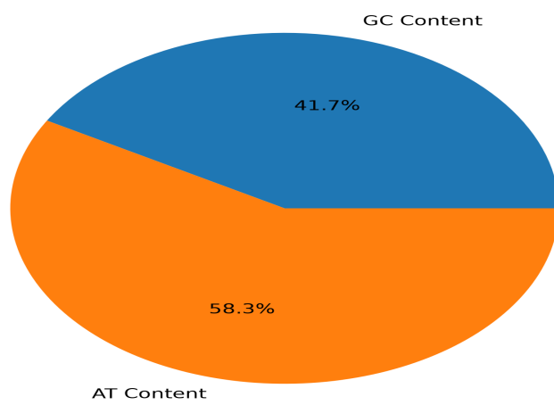
GC vs AT Content
