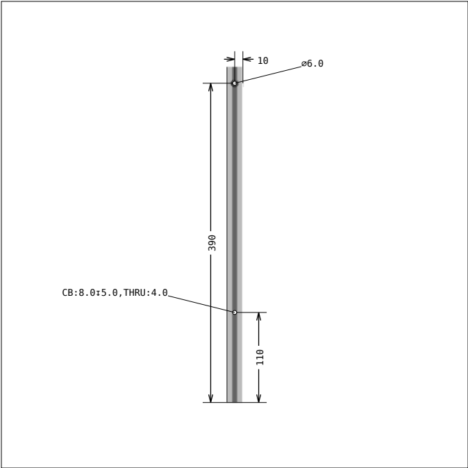
DRAWING 2, Pos 3 SIDE 1, bar length: 410 mm
