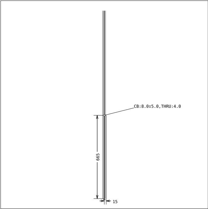
DRAWING 10, Pos 16 SIDE 3
