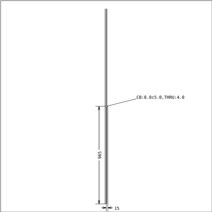
DRAWING 12, Pos 18 SIDE 1, bar length: 1930 mm
