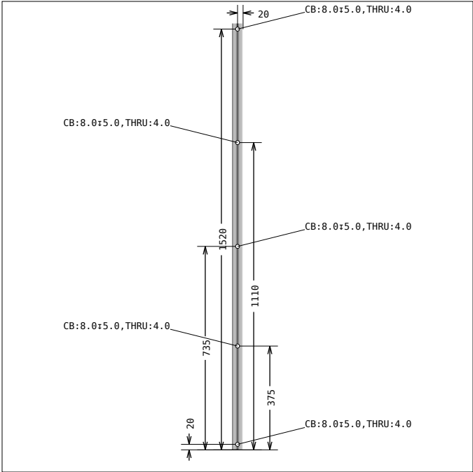
DRAWING 14, Pos 25 SIDE 2
