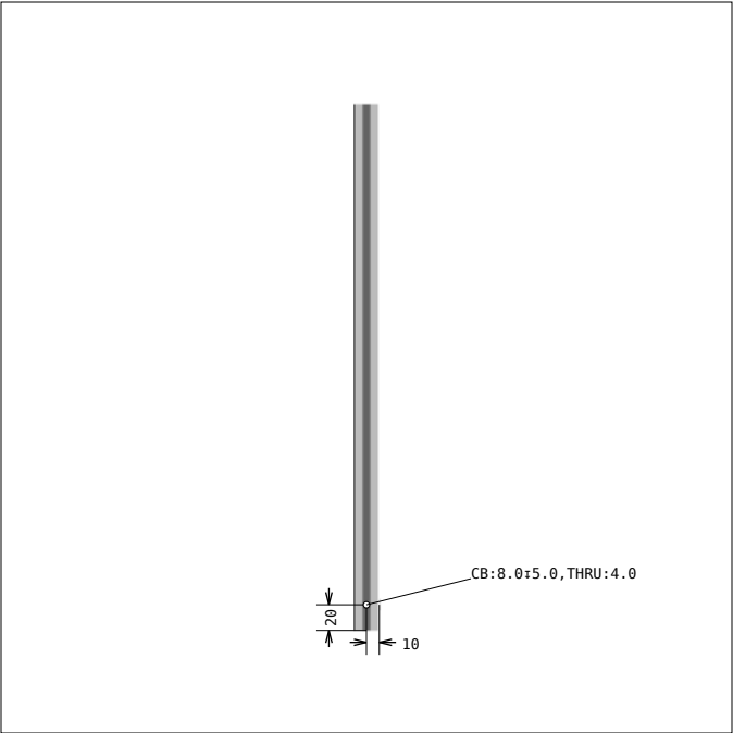
DRAWING 1, Pos 2 SIDE 2
