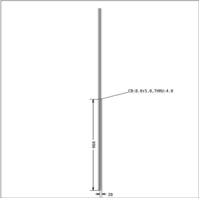
DRAWING 16, Pos 27 SIDE 2
