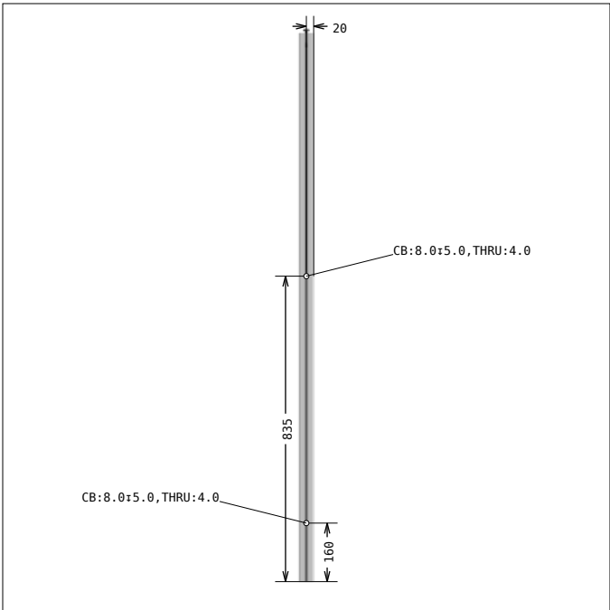
DRAWING 18, Pos 30 SIDE 4
