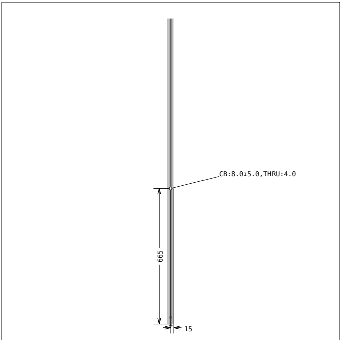
DRAWING 9, Pos 15 SIDE 4
