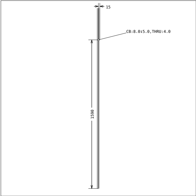
DRAWING 12, Pos 18 SIDE 2
