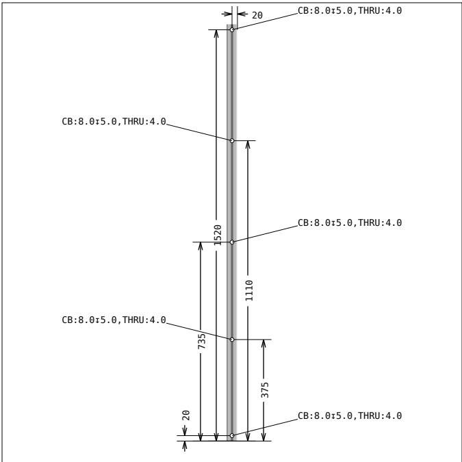
DRAWING 13, Pos 24 SIDE 4
