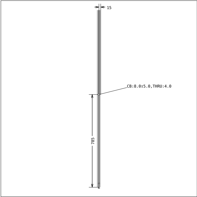
DRAWING 11, Pos 17 SIDE 4
