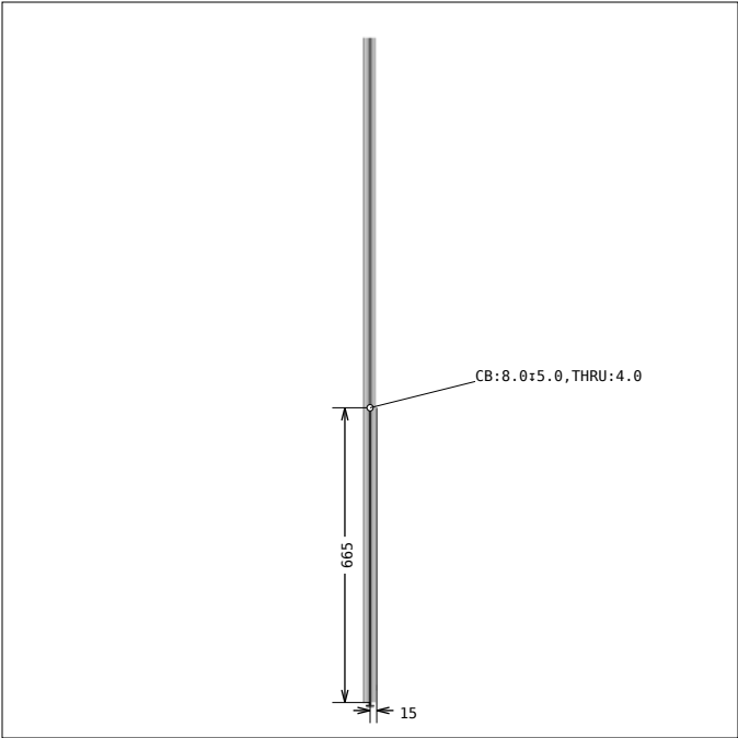
DRAWING 11, Pos 17 SIDE 1, bar length: 1500 mm
