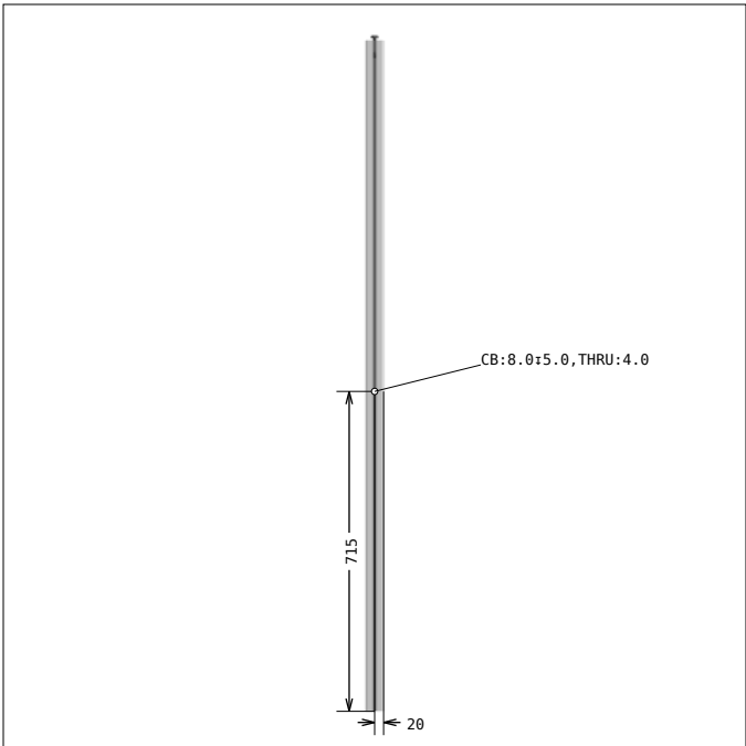
DRAWING 17, Pos 29 SIDE 4
