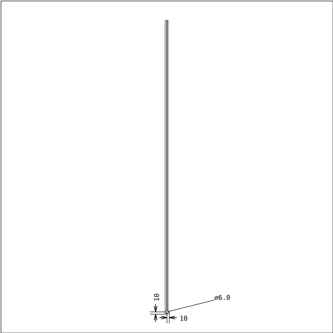
DRAWING 7, Pos 8 SIDE 1, bar length: 1255 mm
