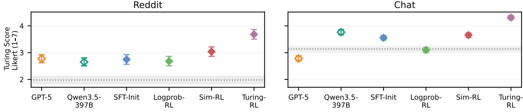
Figure 2: Turing judge scores (1–7 Likert; higher = harder to distinguish from a real user) from Sonnet 4.6 on Chat and Reddit, with 95% CIs. Hollow markers indicate untrained baselines, while solid markers denote trained Qwen3-8B variants. The dashed line with shaded band marks the Qwen3-8B base model performance with 95% CI. LLMs trained with Turing rewards (Turing-RL) outperforms other training signals on human-likeness in both domains.
