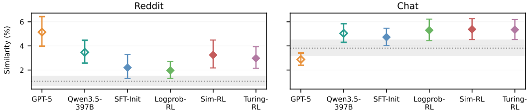
Figure 3: Response similarity to ground truth (Sim, %; higher = more similar to what the user actually said) from Sonnet 4.6 on Chat and Reddit, with 95% CIs. Hollow markers indicate untrained baselines, while solid markers denote trained Qwen3-8B variants. The dashed line with shaded band marks the Qwen3-8B base model performance with 95% CI. Turing-RL matches Sim-RL even though Sim-RL is explicitly trained to maximize similarity, showing that optimizing for indistinguishability does not sacrifice content alignment.
