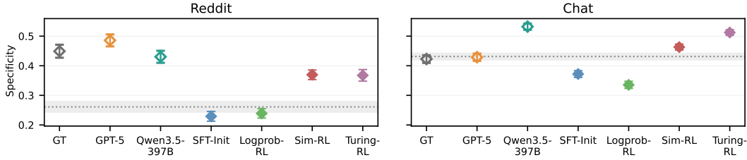
Figure 4: Response specificity ( [0, 1] ; higher = more grounded in the interaction context and compatible with the target user) from Sonnet 4.6, with 95% CIs. Hollow markers indicate untrained baselines, while solid markers denote trained Qwen3-8B variants. GT is the ground truth human response, and the dashed line marks the Qwen3-8B base model with 95% CI. Turing-RL is among the strongest on Chat, while Turing-RL and Sim-RL are strongest among the trained models on Reddit , outperforming SFT-Init and Logprob-RL.
