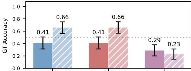
Reddit
