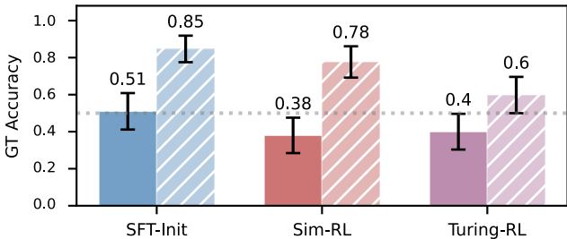
Reddit
