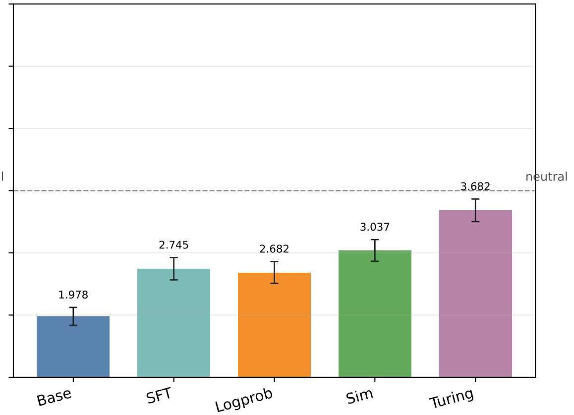
Reddit
