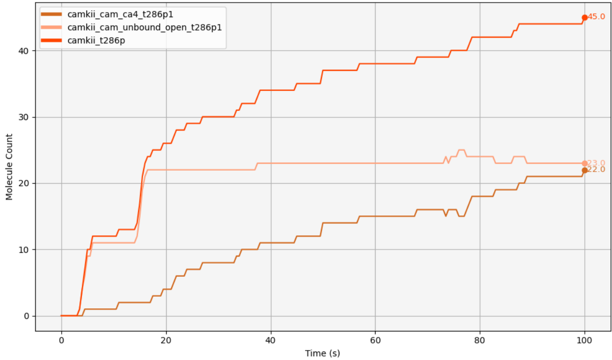
Figure 6.8: CaM binding is not the main event leading to the increase of initial CaMKII T286 phosphorylation, as out of all the CaMKII that is T286 phosphorylated (camkii_t286p), most of it first increases in a state that is free from CaM (camkii_cam_unbound_open_t286p1), whereas CaMKII that is bound to CaM and T286 phosphorylated (camkii_cam_ca4_t286p1) increases more slowly and later.
