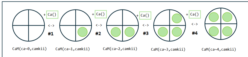
Figure 5.5: We model calcium binding to CaM following “scheme 3” proposed by Linkevicius et al., 2024 [456]. It is a sequential CaM scheme where each binding site is represented individually.
