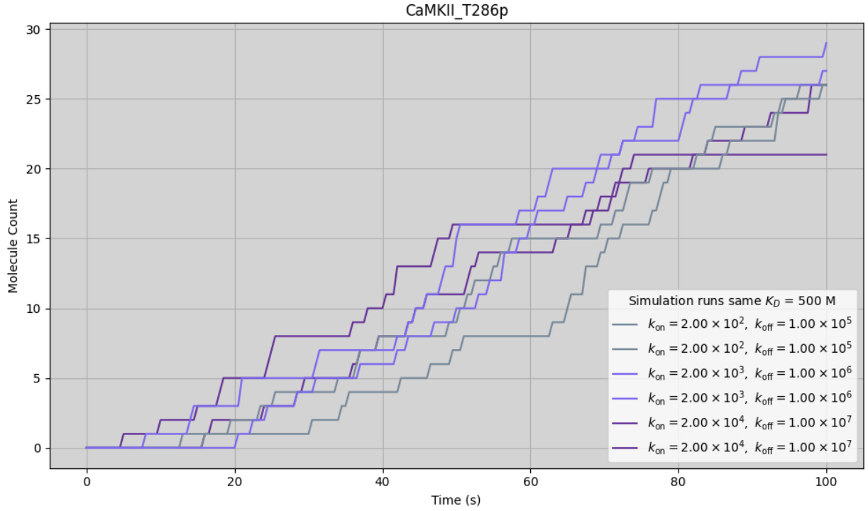
Figure 5.7: CaMKII T286 phosphorylation was unaffected by changes in k_{\text{on}} and k_{\text{off}} by factors of 0.1 and 0.01. The baseline values for k_{\text{on}} and k_{\text{off}} were taken from [185]: k_{\text{off}} = 1.00 \times 10^7 \text{ s}^{-1} and k_{\text{on}} = 2.00 \times 10^4 \text{ M}^{-1}\text{s}^{-1} . Simulations were performed by varying these parameters by factors of 0.1 and 0.01, with the equilibrium dissociation constant ( k_D ) held constant at 500 M.
