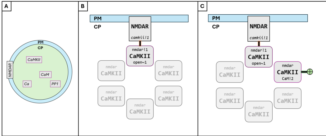
Figure 5.3: Simplified schematic of CaMKII binding to NMDARs in Compartmental BioNetGen. (A) A cell is defined with plasma membrane (PM) and cytoplasm (CP) volumes. Molecules are released as surface molecules (NMDARs) or volume molecules (rest). (B) NMDARs embedded in the PM can bind to CaMKII subunits diffusing within the cytoplasm. (C) Different subunits within the CaMKII dodecamer (simplified here as a hexamer) can independently interact with other molecules such as NMDAR or CaM. These interactions can occur simultaneously or asynchronously, allowing CaMKII to integrate multiple signals through subunit-specific states.
