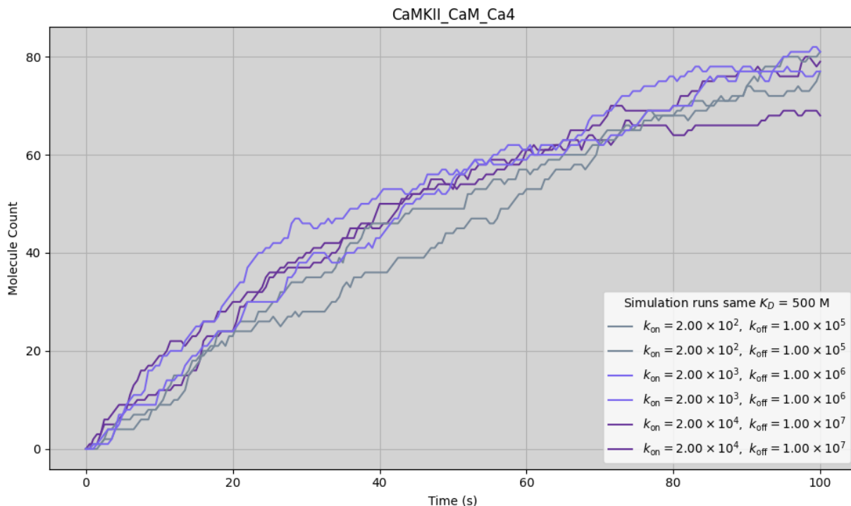
Figure 5.8: CaMKII binding to CaM was unaffected by changes in k_{\text{on}} and k_{\text{off}} by factors of 0.1 and 0.01. The baseline values for k_{\text{on}} and k_{\text{off}} were taken from [185]: k_{\text{off}} = 1.00 \times 10^7 \text{ s}^{-1} and k_{\text{on}} = 2.00 \times 10^4 \text{ M}^{-1}\text{s}^{-1} . Simulations were performed by varying these parameters by factors of 0.1 and 0.01, with the equilibrium dissociation constant ( k_{\text{D}} ) held constant at 500 M.
