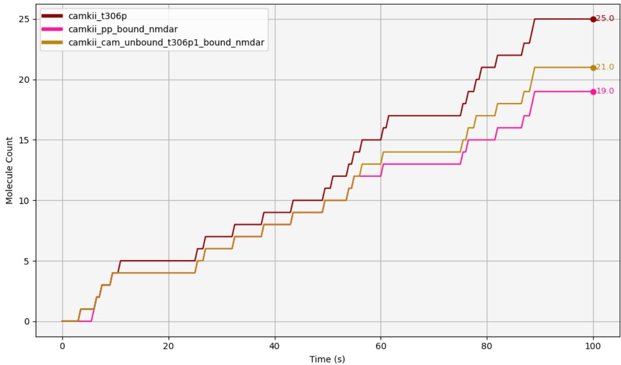
Figure 6.10: At later stages, T306 phosphorylation can occur and persist independently of T286 in CaMKII that is bound to NMDARs. Initially, most of the CaMKII phosphorylated at T306 ( camkii_t306p ) is also phosphorylated at T286—i.e., it is in the doubly phosphorylated state ( camkii_pp_bound_nmdar ). This indicates that early T306 phosphorylation often coincides with T286 phosphorylation. After 60 seconds, the amount of CaMKII that is bound to NMDARs and phosphorylated only at T306 ( camkii_cam_unbound_t306p1_bound_nmdar ) surpasses the doubly phosphorylated form . Saying cam_unbound (CaM free) in this molecule name is redundant as camkii that is t306p is necessarily free from CaM.
