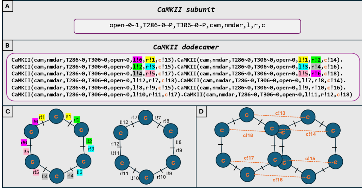
Figure 5.2: (A) The open flag determines whether the subunit is in a closed (0) or open (1) state. The T286 and T306 flags represent the phosphorylation states, where a value of 0 indicates the subunit is unphosphorylated, and “P” indicates phosphorylation. The cam flag refers to a binding site for CaM, which can either be bound or unbound. Similarly, the nmdar flag represents another binding site for the NMDA receptor, which can also be in a bound or unbound state. The cam and nmdar flags represent binding events that can occur or not, depending on whether CaM or NMDA receptors are bound to the subunit. (B) The left (l), right (r), and centre (c) binding sites facilitate the assembly of subunits into two hexameric rings. These rings are stabilised via interactions at the centre binding site. Subunits participating in the left and right rings are highlighted in matching colours to distinguish the respective assemblies. (C) A more visual depiction of the two separated hexameric rings. (D) The centre binding interactions are specifically highlighted to show the dodecameric representation of CaMKII in the model.
