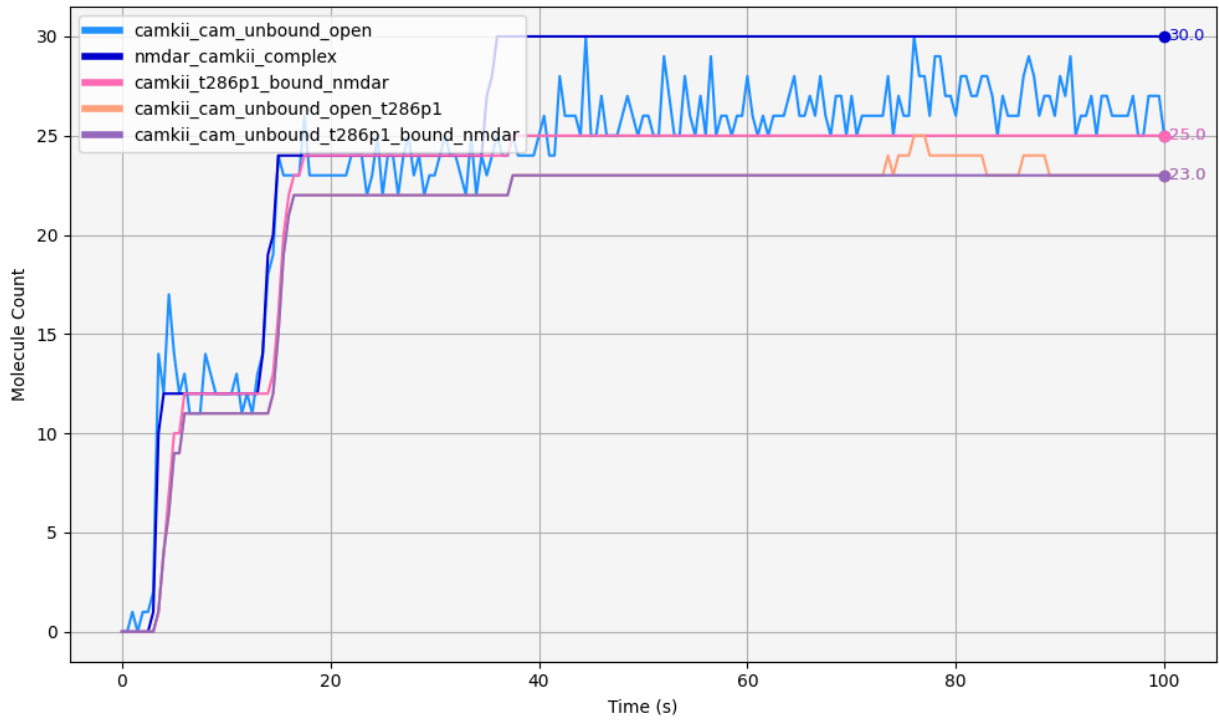
Figure 6.9: Binding of CaMKII to NMDARs promotes and stabilizes the open conformation of its subunits, facilitating T286 autophosphorylation within the CaMKII/NMDAR complex.
