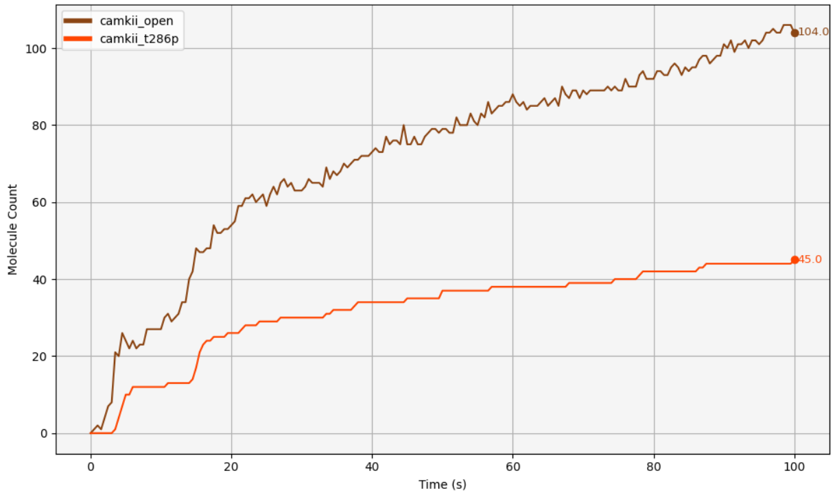
Figure 6.5: Approximately half of CaMKII that is open (camkii_open) is also phosphorylated at T286 (camkii_t286p). The difference between 104 and 45 is the amount of CaMKII that is open and unphosphorylated at T286.
