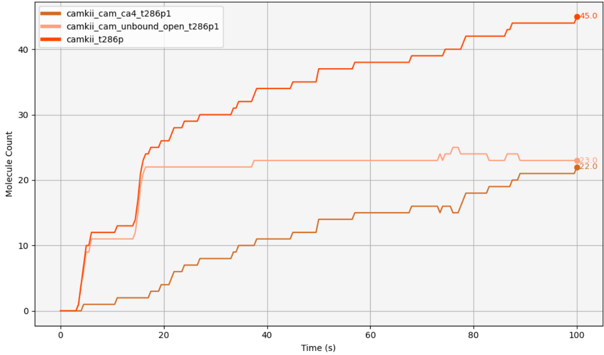
Figure 6.8: CaM binding is not the main event leading to the increase of initial CaMKII T286 phosphorylation, as out of all the CaMKII that is T286 phosphorylated (camki_t286p), most of it first increases in a state that is free from CaM (camkii_cam_unbound_open_t286p1), whereas CaMKII that is bound to CaM and T286 phosphorylated (camkii_cam_ca4_t286p1) increases more slowly and later.
