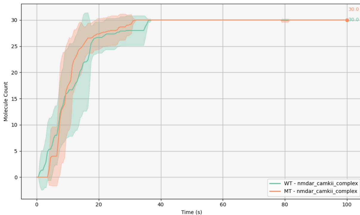
Figure 6.17: NMDAR binding reaches full saturation in both WT and NMDAR/CaMKII mutant models. Shaded areas indicate the standard deviation. Both models ultimately reach a plateau of 30 bound CaMKII/NMDAR complexes. Due to the lack of variability in the final molecule count (both reach 30 with no variance), statistical comparisons of the end-point data are not shown.
