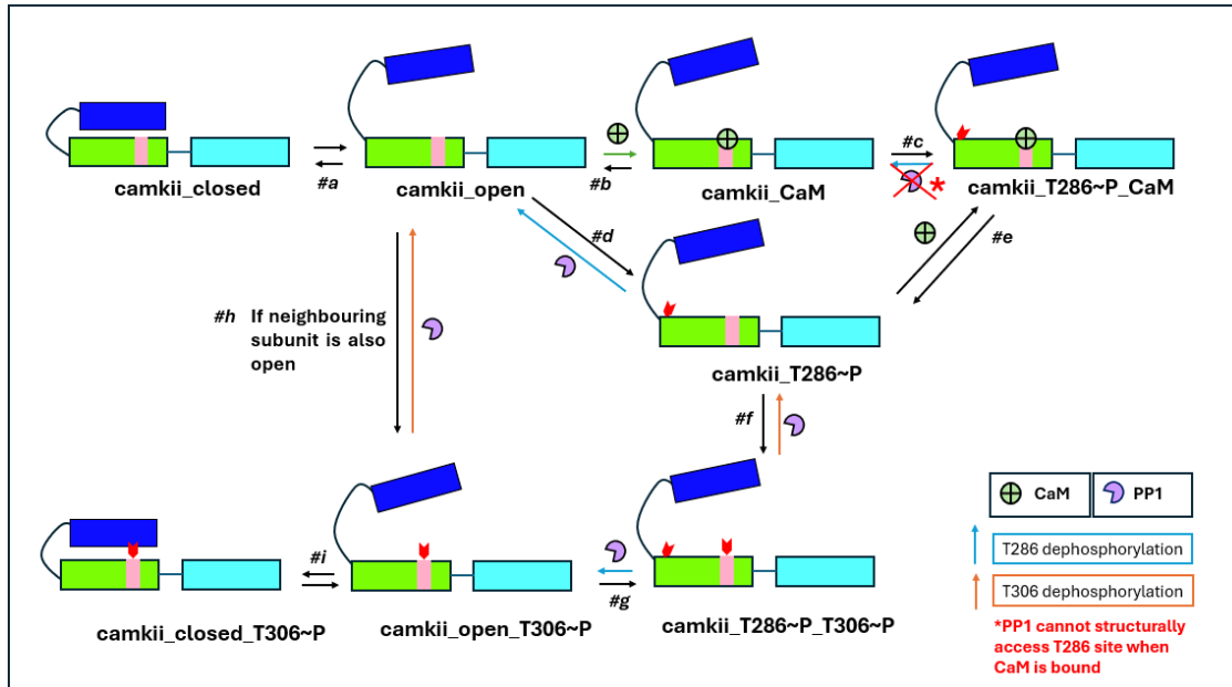
Figure 5.6: Reaction rules depicted for possible reaction pathways of CaMKII subunits. (#a) CaMKII in a closed state can flicker between open and closed states; (#b) CaMKII that is open can reversibly bind to a CaM molecule; (#c) CaMKII that is bound to CaM can phosphorylate at T286 (T286~P), and if CaM is bound, PP1 cannot structurally access the subunit to dephosphorylate it; (#d) CaMKII that is open and free from CaM can also phosphorylate at T286, and PP1 can access and dephosphorylate it in this state; (#e) CaMKII that is bound to CaM and T286~P can release CaM and remain T286P; (#f) CaMKII T286~P can also phosphorylate at T306, and PP1 can dephosphorylate the T306 site as well; (#g) When CaMKII is phosphorylated at both sites, PP1 can also dephosphorylate T286 instead of T306, and CaMKII that is T306P can also autophosphorylate at T286; (#h) CaMKII that is T306P can be dephosphorylated by PP1, and if a CaMKII subunit that is open has a neighbouring subunit that is also open, it may autophosphorylate at T306; (#i) CaMKII that is T306P can close (unlike when CaMKII is T286~P).
