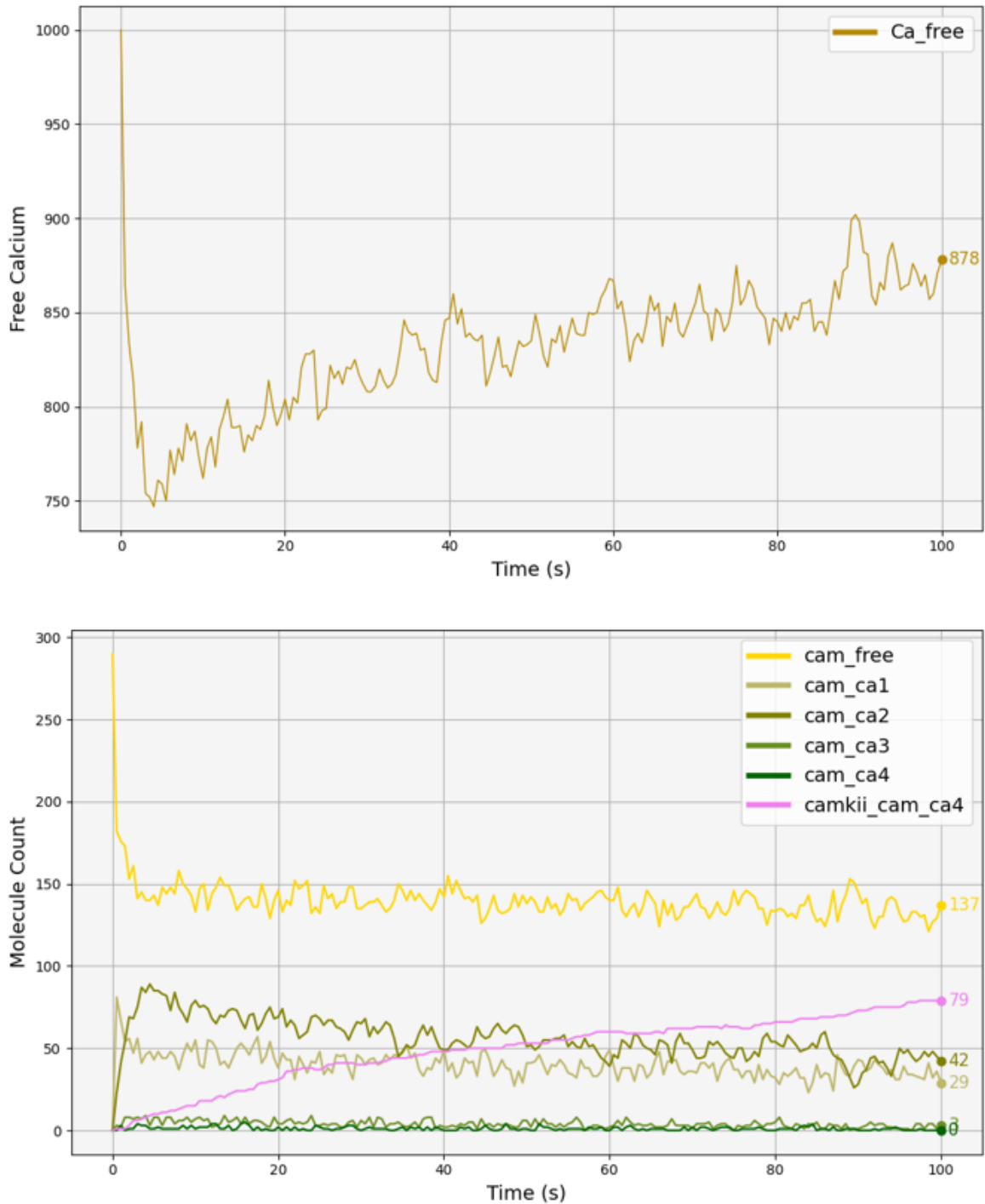
Figure 6.3: CaM binding to 1,2,3 and 4 calcium ions (calcium not shown) and formation of CaMKII-CaM complex (CaMKII_CaM_Ca4).
