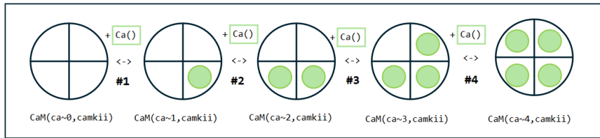
Figure 5.4: We model calcium binding to CaM following “scheme 3” proposed by Linkevicius et al., 2024. It is a sequential CaM scheme where each binding site is represented individually.
