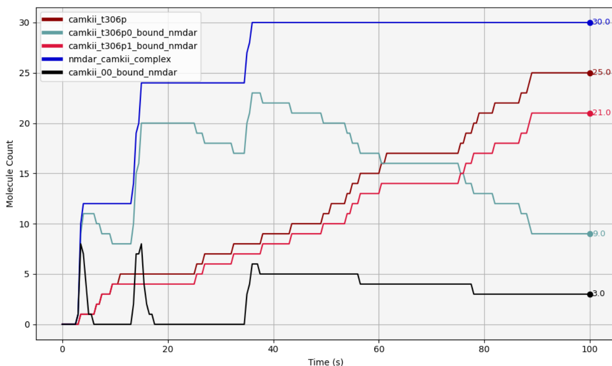
Figure 6.11: CaMKII binds unphosphorylated to NMDARs ( camkii_00_bound_nmdar ). T286 phosphorylation ensues, followed by an increase in T306 phosphorylation ( camkii_t306p1_bound_nmdar ) -and a T306 unphosphorylated state decrease ( camkii_t306p0_bound_nmdar ). All these molecules are a subset of CaMKII bound to NMDARs ( nmdar_camkii_complex ).
