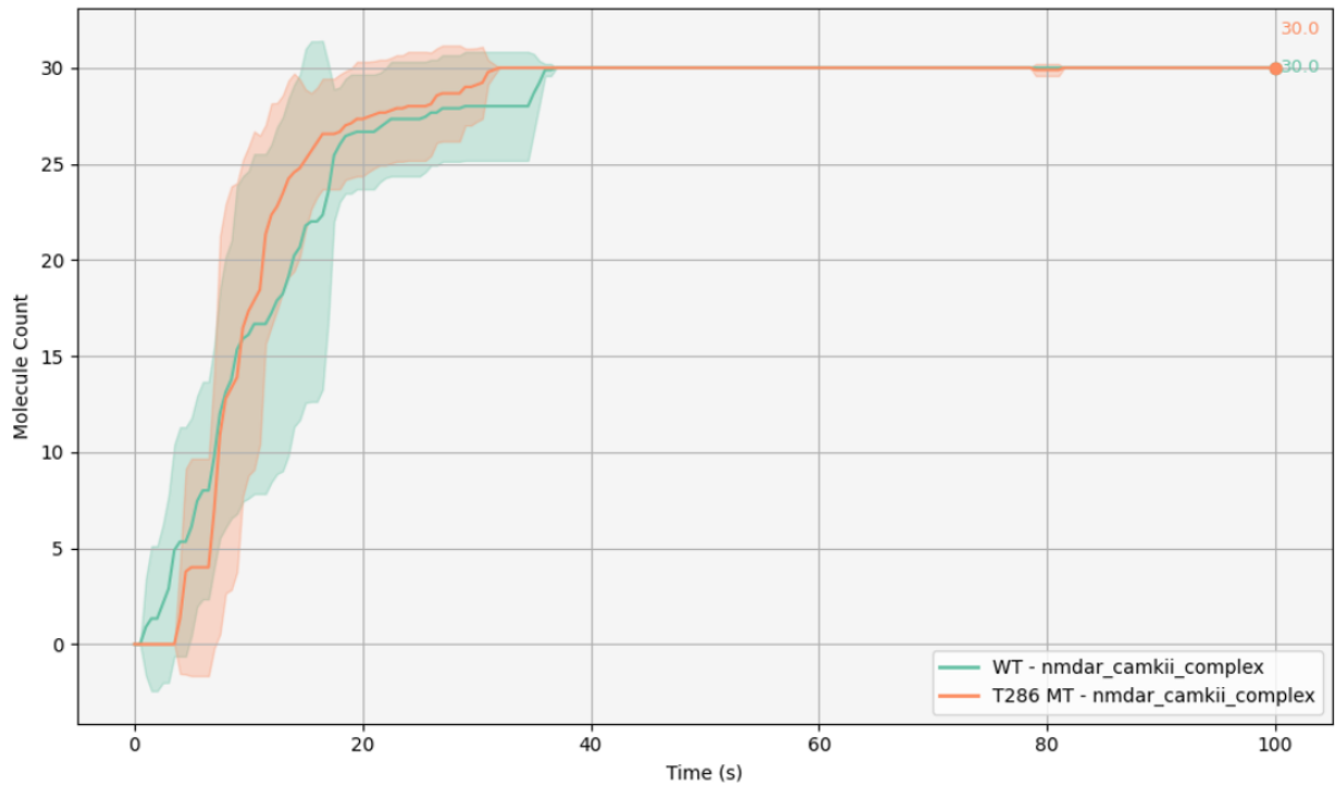
Figure 6.17: Lack of T286 phosphorylation does not seem to influence the binding of CaMKII to NMDARs. NMDAR binding reaches full saturation in both WT and T286 mutant models. Shaded areas indicate the standard deviation. Both models ultimately reach a plateau of 30 bound CaMKII/NMDAR complexes. Due to the lack of variability in the final molecule count (both reach 30 with no variance), statistical comparisons of the end-point data are not shown.
