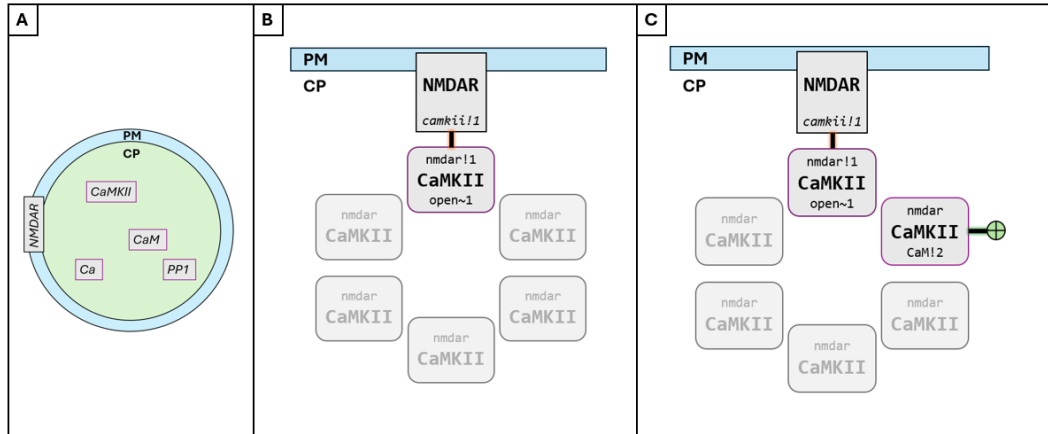
Figure 5.3: Simplified schematic of CaMKII binding to NMDARs in Compartmental BioNetGen. (A) A cell is defined with plasma membrane (PM) and cytoplasm (CP) volumes. Molecules are released as surface molecules (NMDARs) or volume molecules (rest). (B) NMDARs embedded in the PM can bind to CaMKII subunits diffusing within the cytoplasm. (C) Different subunits within the CaMKII dodecamer (simplified here as a hexamer) can independently interact with other molecules such as NMDAR or CaM. These interactions can occur simultaneously or asynchronously, allowing CaMKII to integrate multiple signals through subunit-specific states.
