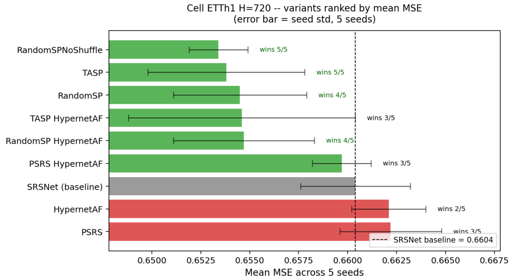
Figure 6: ETTh1 H=720 – mean MSE across 5 seeds, ranked ascending. Two variants beat the baseline on 5/5 seeds: RandomSPNoShuffle (−1.07%) and TASP (−1.00%). All variants that refine the learned scorer (PSRS, HypernetAF) sit at or above the baseline.
