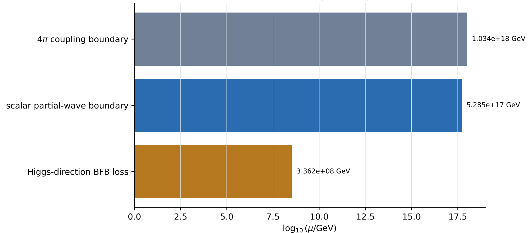
Point-matched leading one-loop scales
