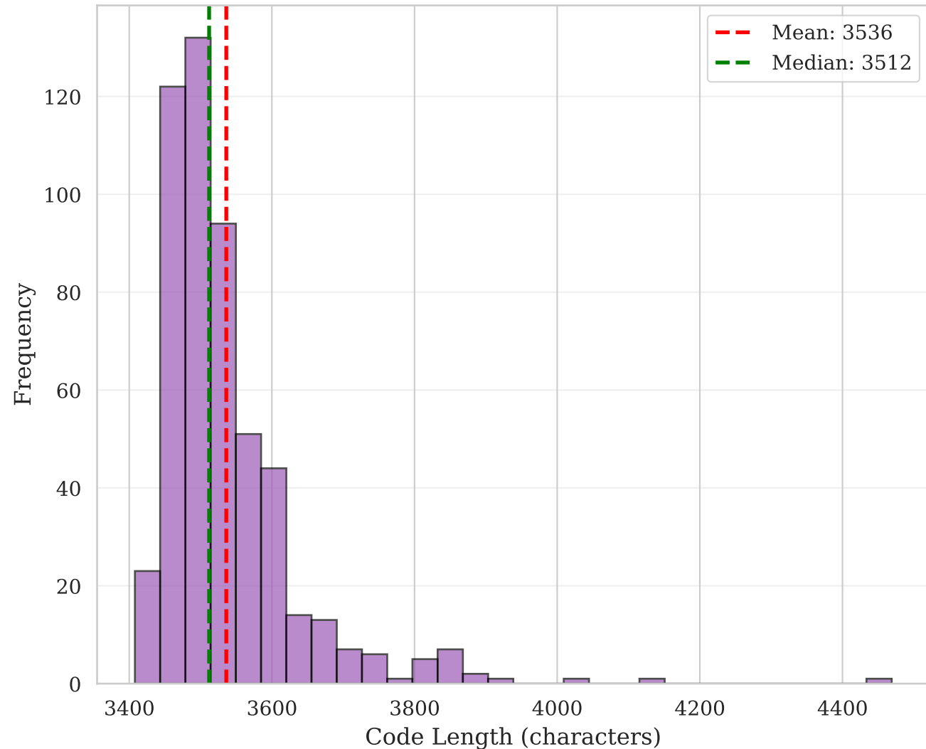
Distribution of Generated Code Length
