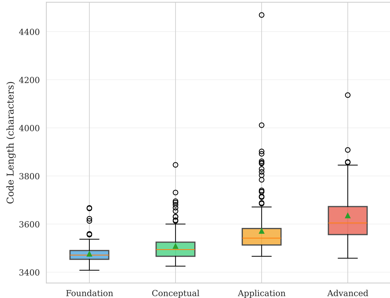
Code Length by Curriculum Level
