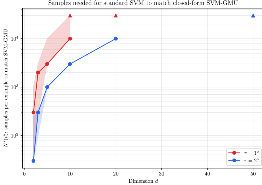
Figure 9: Samples-to-match N^*(d) versus dimension d on a logarithmic vertical axis, for tolerances \tau = 1^\circ and \tau = 2^\circ . Solid markers are the median over R = 30 seeds and the shaded bands span the 25th to 75th percentile. Upward triangles at the ceiling mark dimensions where some seeds never reach the tolerance within N_{\max} = 3 \times 10^4 . N^*(d) grows by roughly an order of magnitude per doubling of d , while the closed-form SVM-GMU pays nothing.
