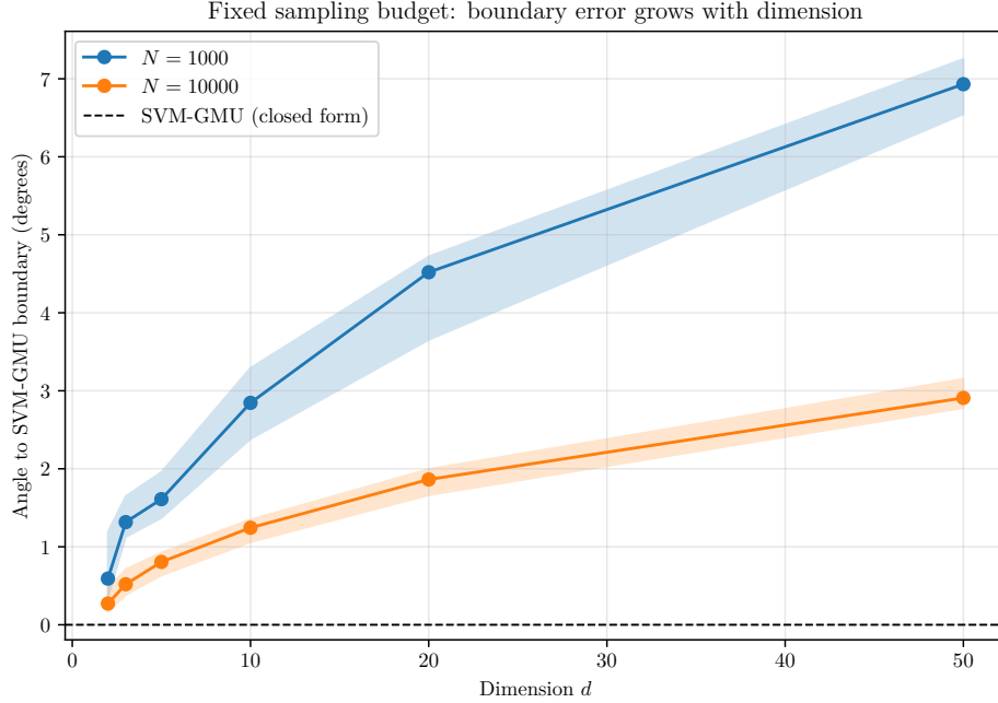
Figure 10: Fixed-budget view: median angle (over R = 30 seeds) between the standard-SVM-on-samples boundary and the closed-form SVM-GMU reference, as a function of dimension d , at two sample budgets N . The dashed line at 0^\circ is the closed-form SVM-GMU, exact at every dimension. At a fixed budget the sampling error grows steadily with d .
