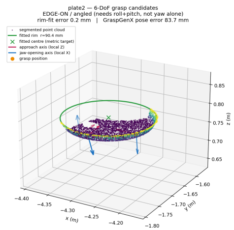
Plate - edge-on, needs roll+pitch
