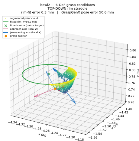
Bowl - top-down straddle
