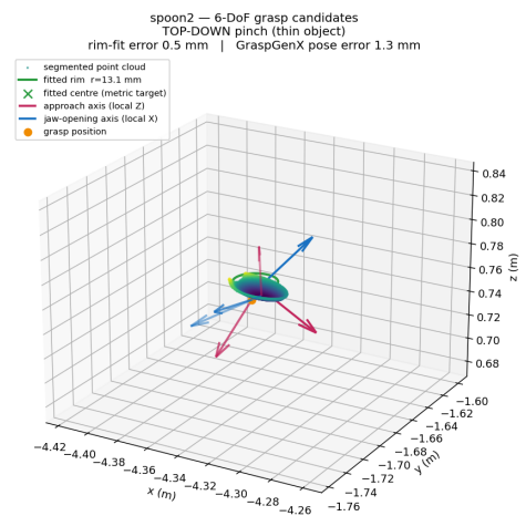
Spoon - top-down pinch
