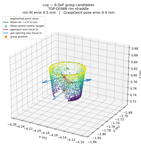
Cup - top-down straddle
