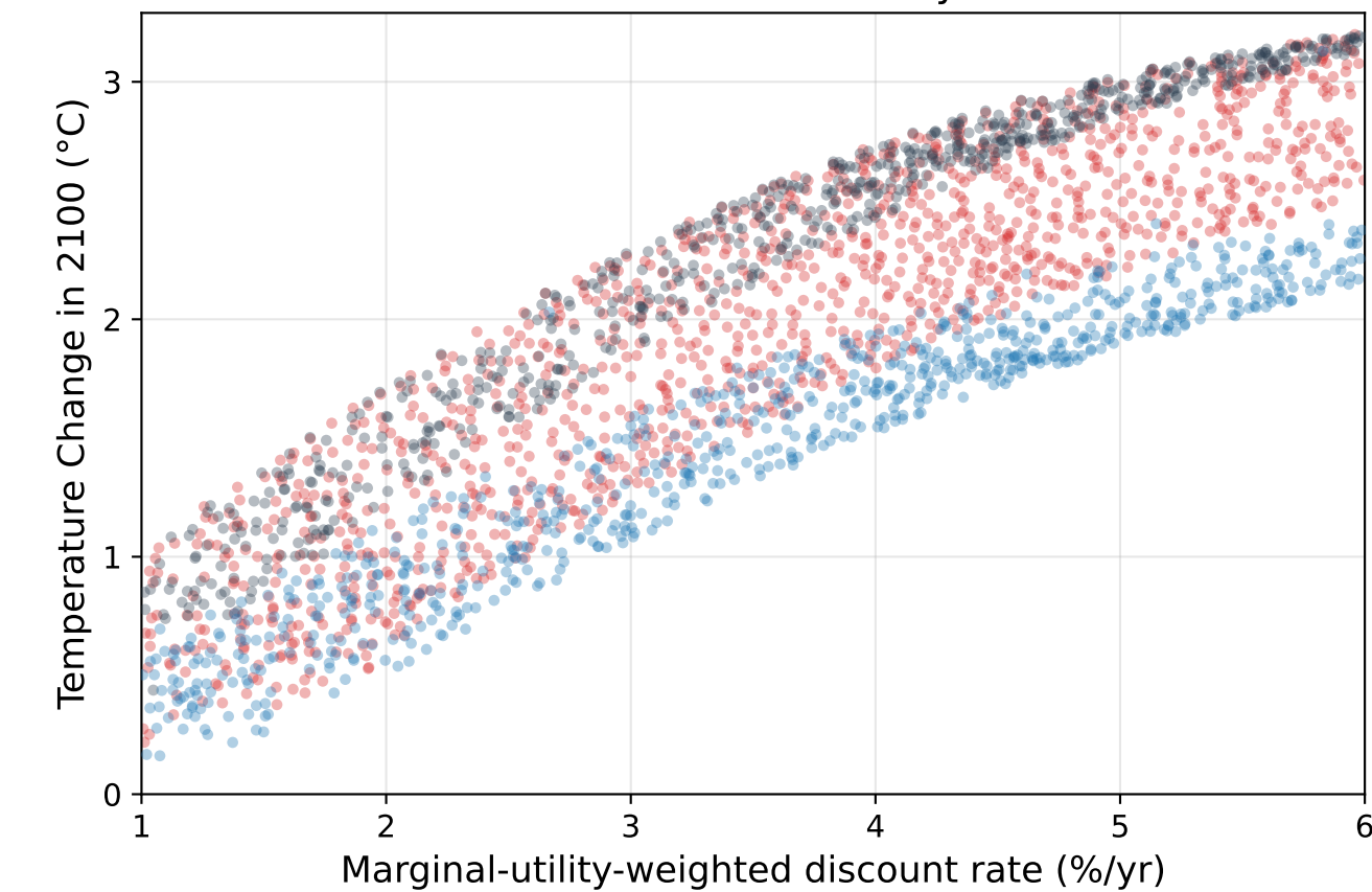
Uniform vulnerability
