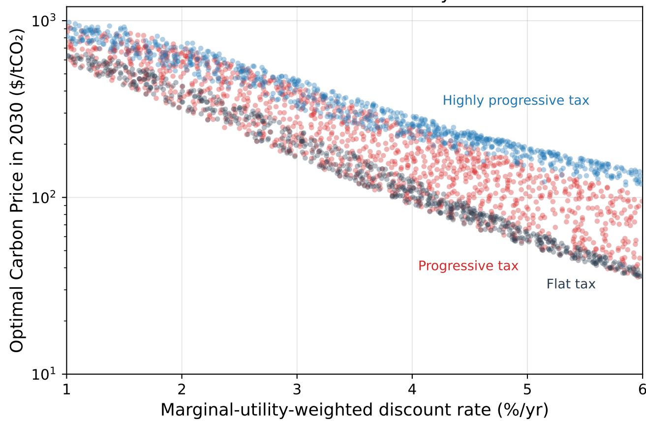
Uniform vulnerability
