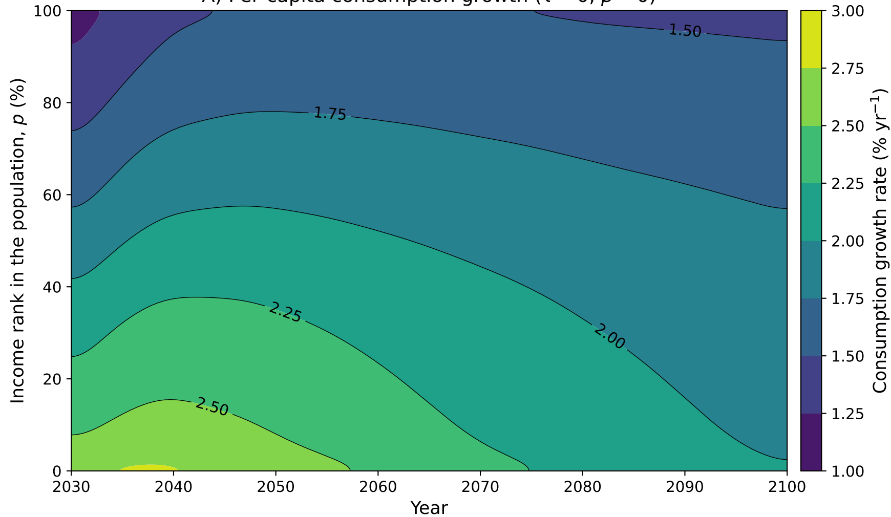
A) Per-capita consumption growth ( \tau = 0 , \beta = 0 )
