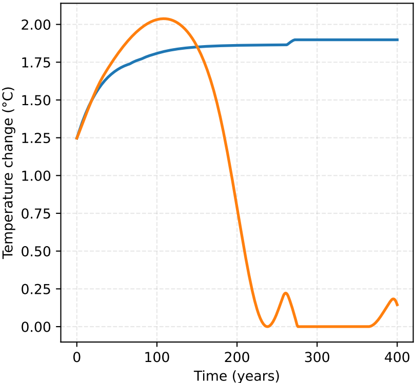
delta_T: Temperature Change from Pre-Industrial
