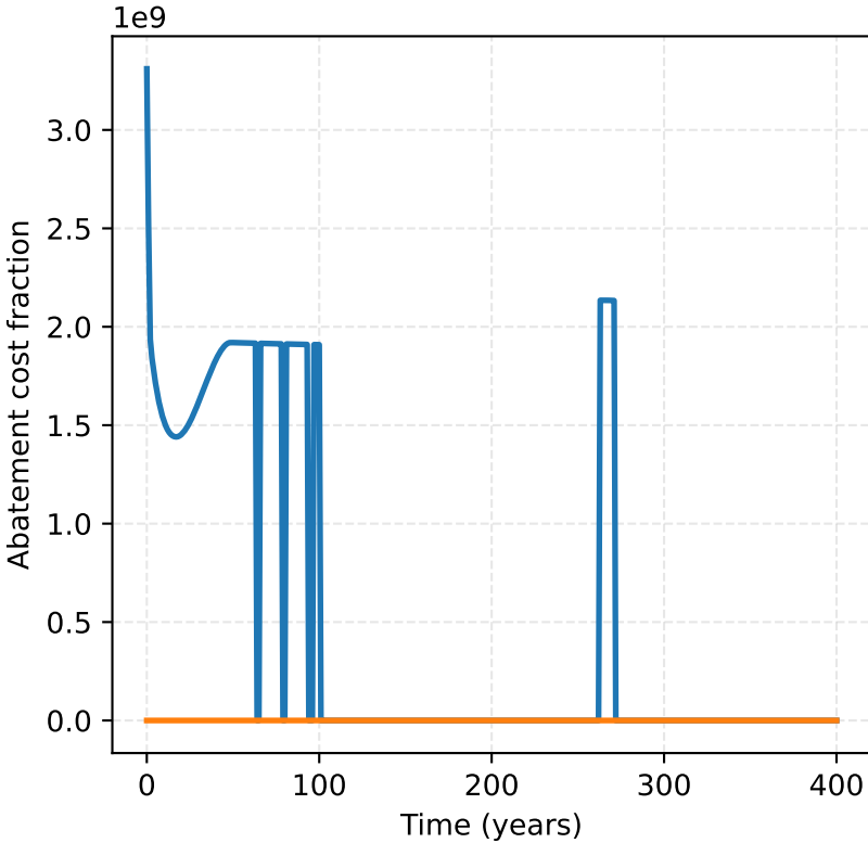
Lambda: Abatement Cost (% of Output)
