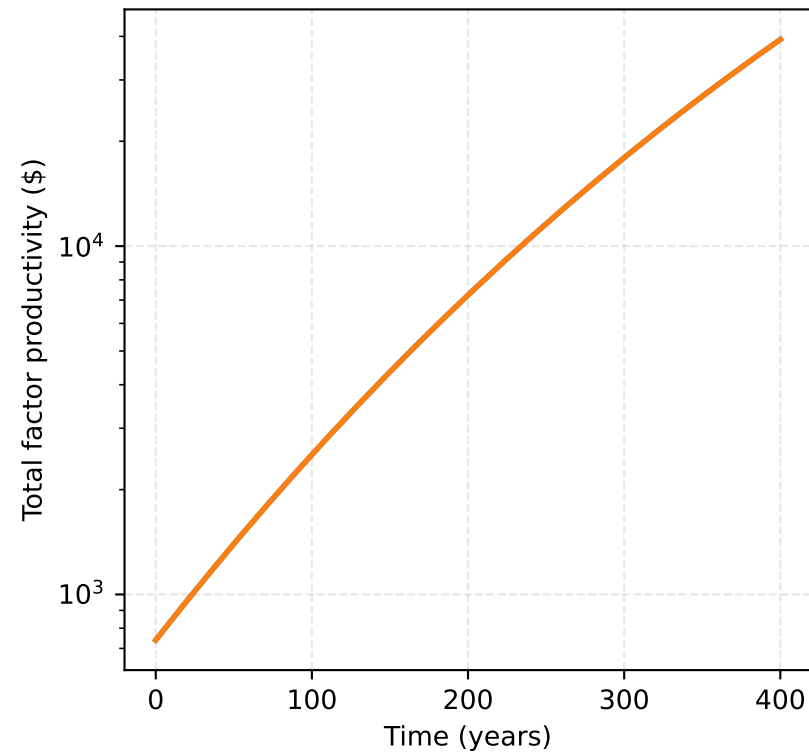
A: Total Factor Productivity
