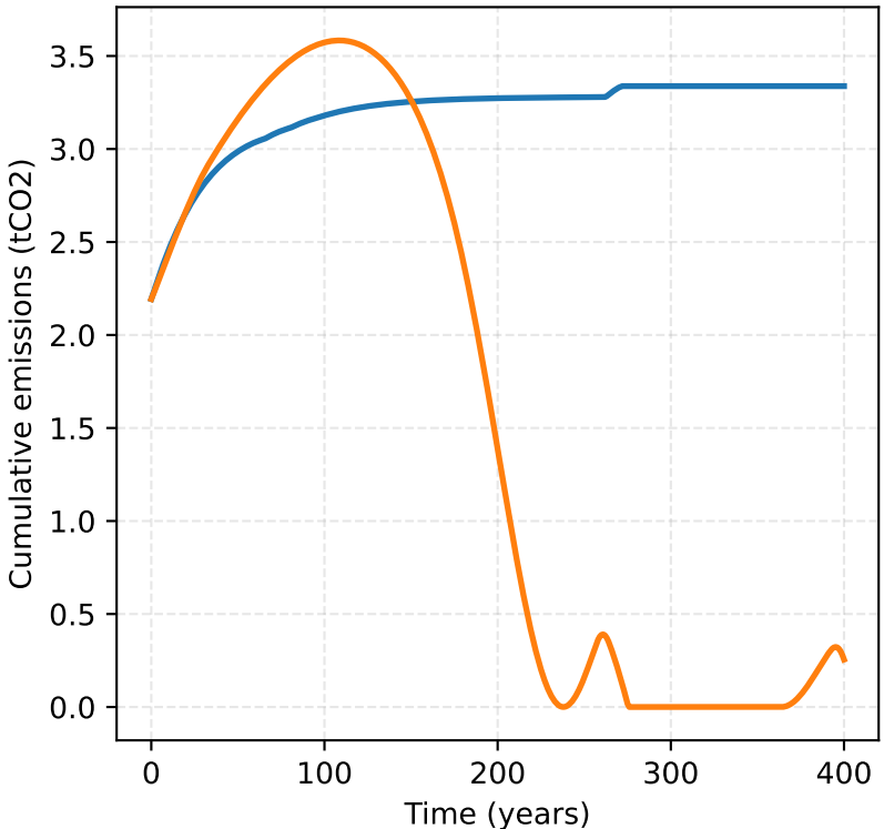
Ecum: Cumulative CO 2 Emissions
