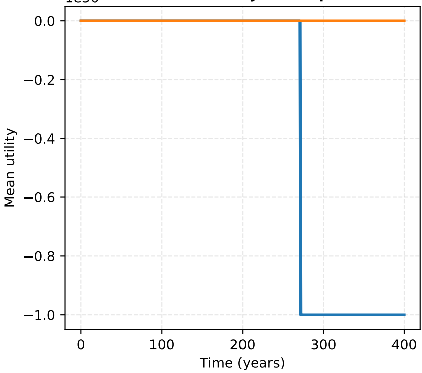
U: Mean Utility Per Capita
