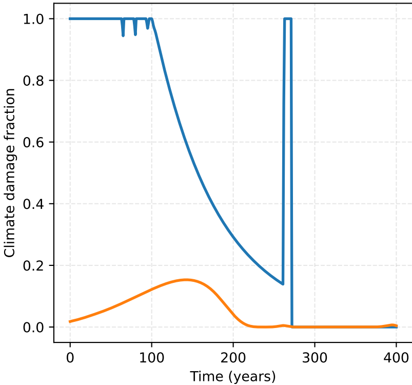
Omega: Climate Damage (% of Output)
