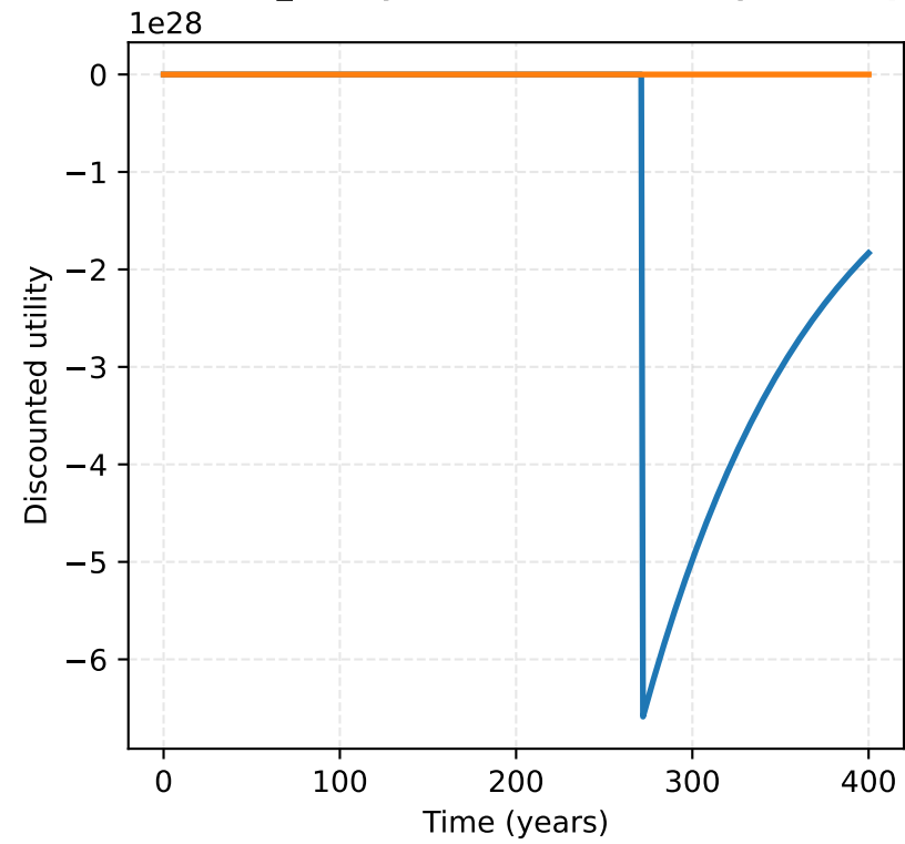
discounted_utility: Discounted Utility Per Capita
