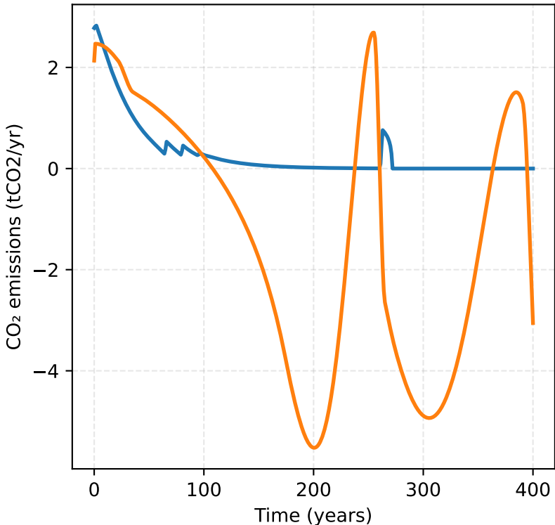
E: CO 2 Emissions Rate
