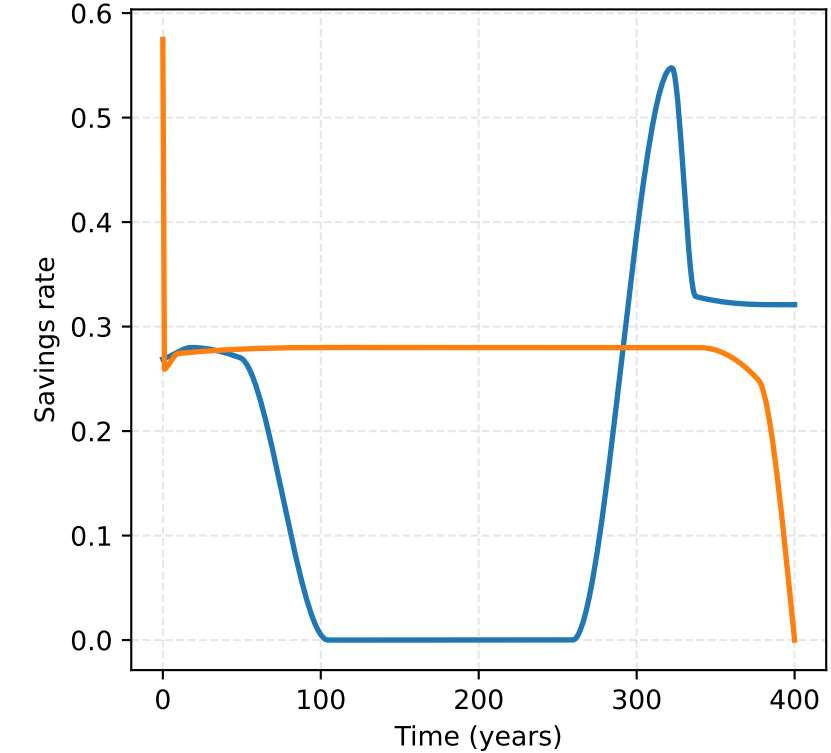
s: Savings Rate Over Time
