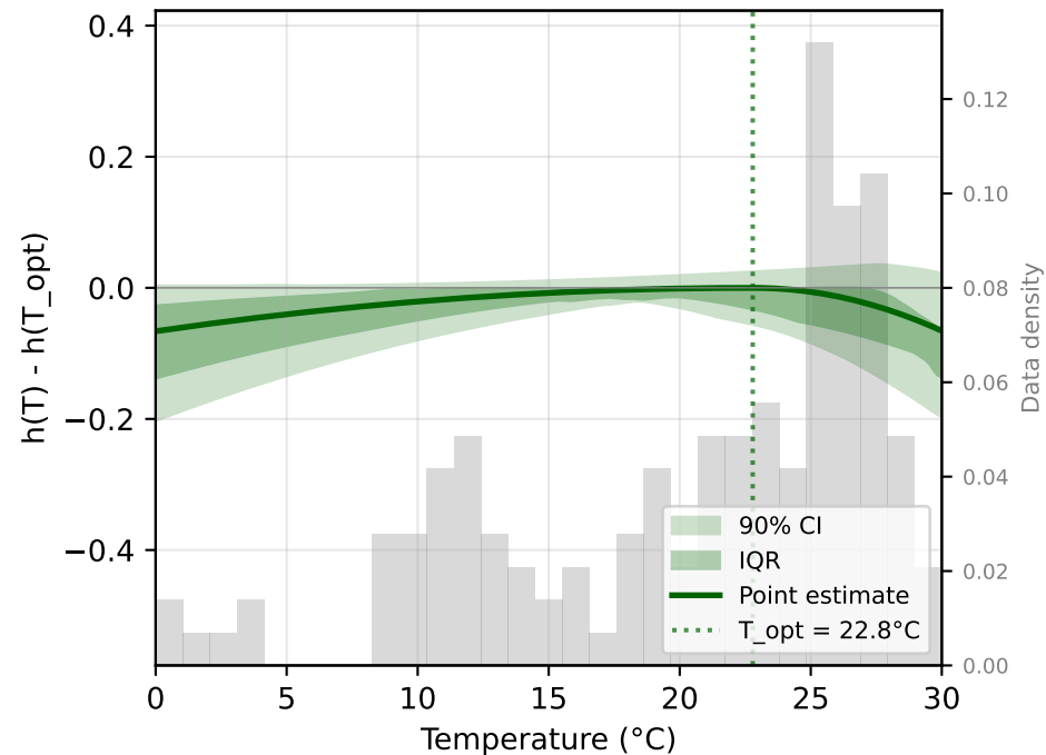
Approach PJ: Piecewise (Joint OLS)
