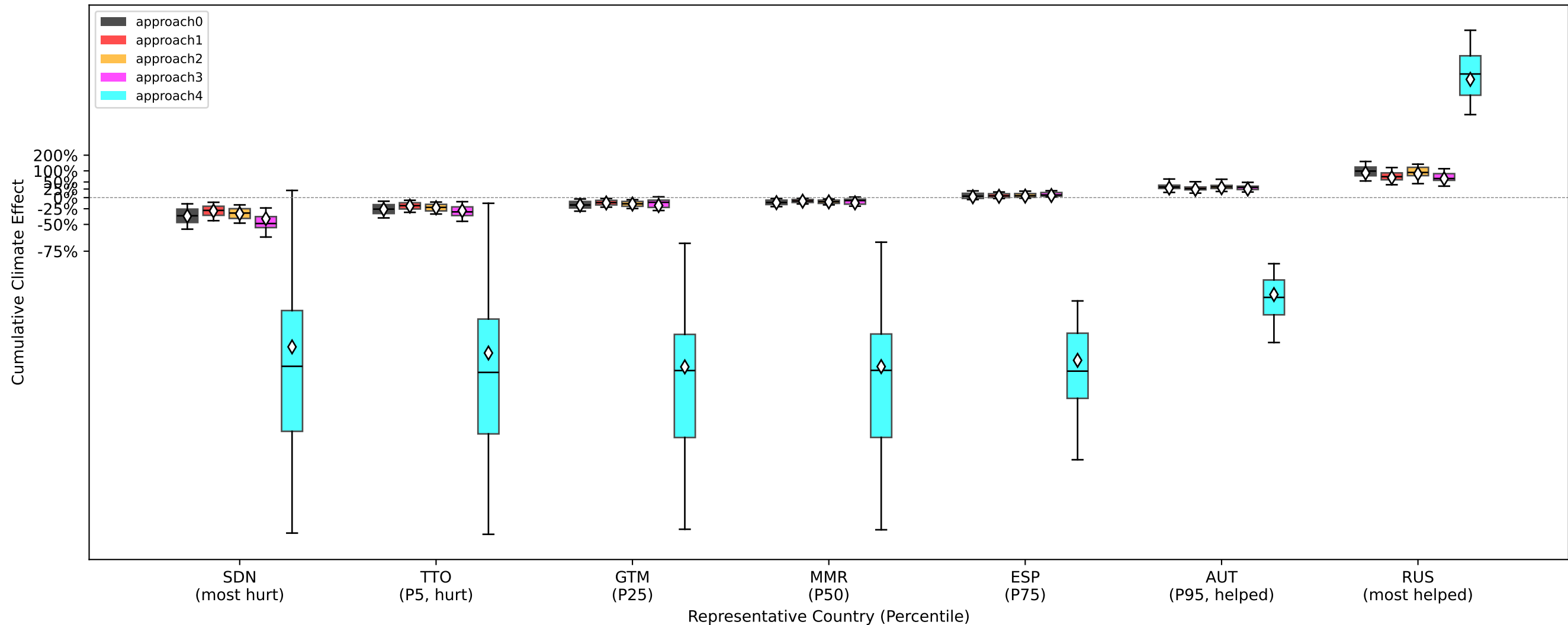
Cumulative Climate Effect on GDP Growth (1961-2022)
