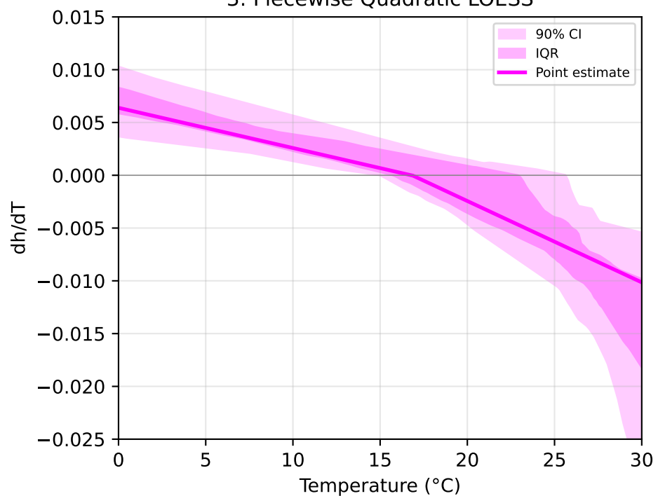
3: Piecewise Quadratic LOESS
