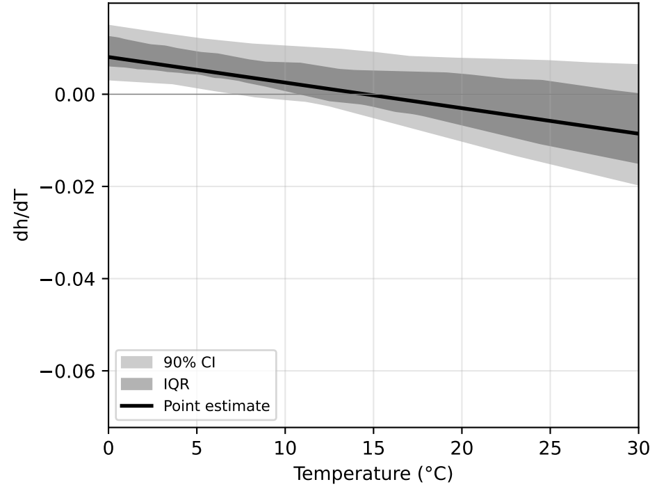
Approach QL: Quadratic (LOESS Detrending)
