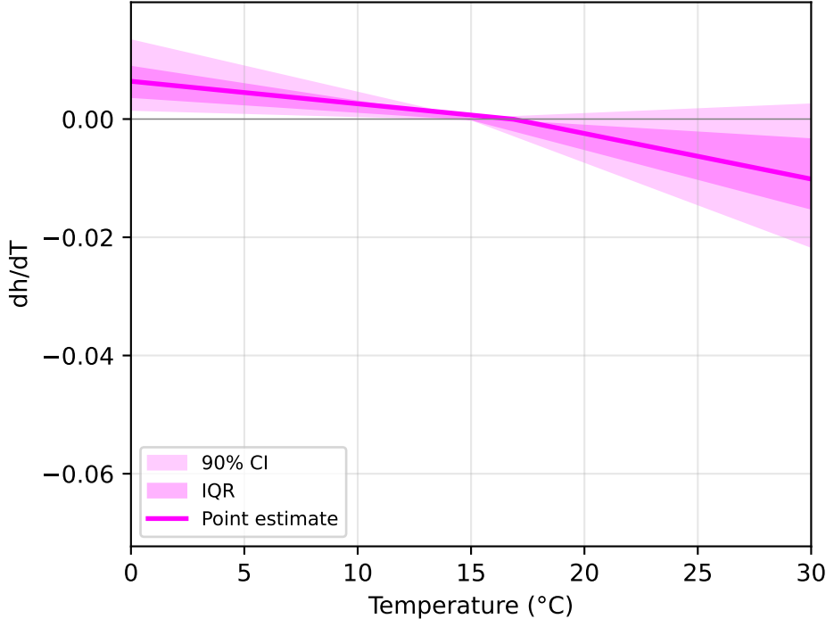
Approach PJ: Piecewise (Joint OLS)
