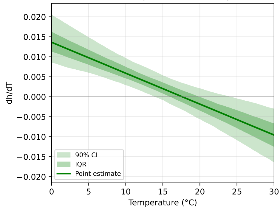
5a: Precomputed k Linear Temp
