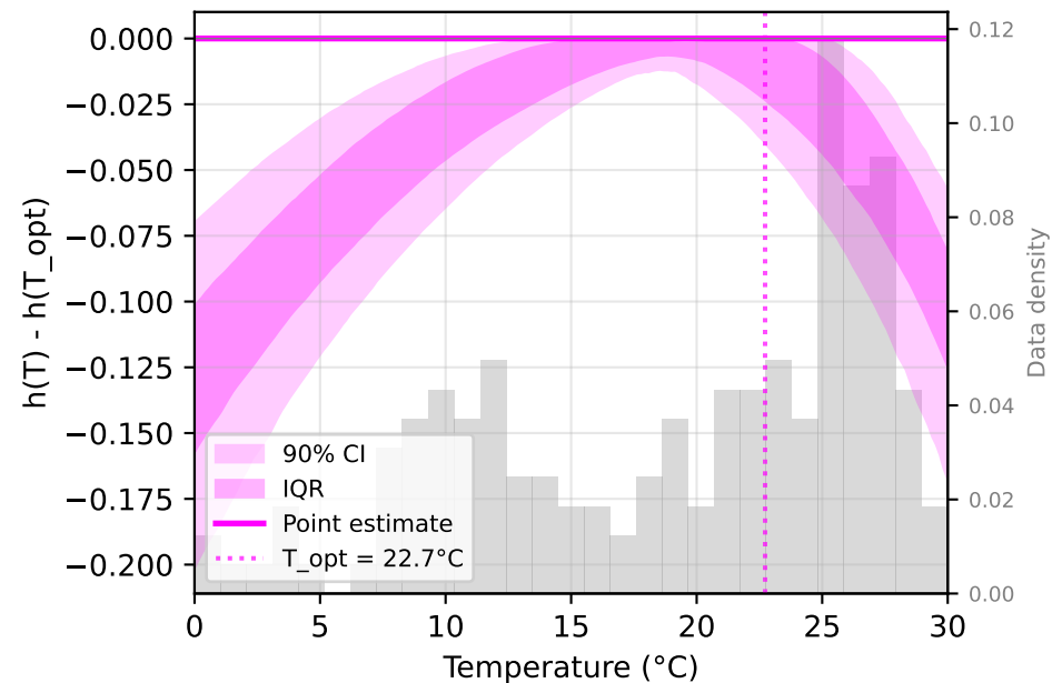
8: Piecewise Quadratic LOESS
