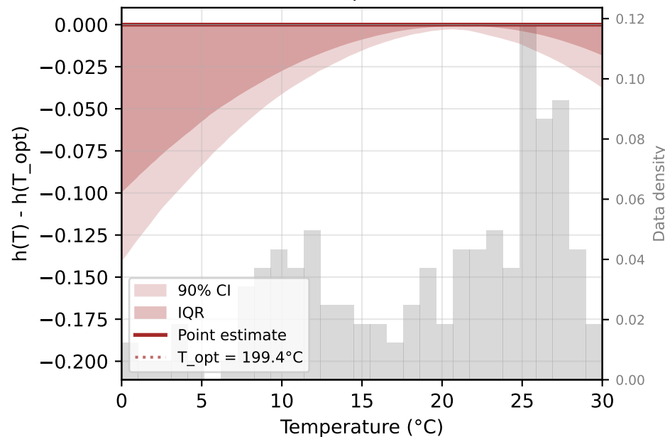
7: GDP-Response LOESS
