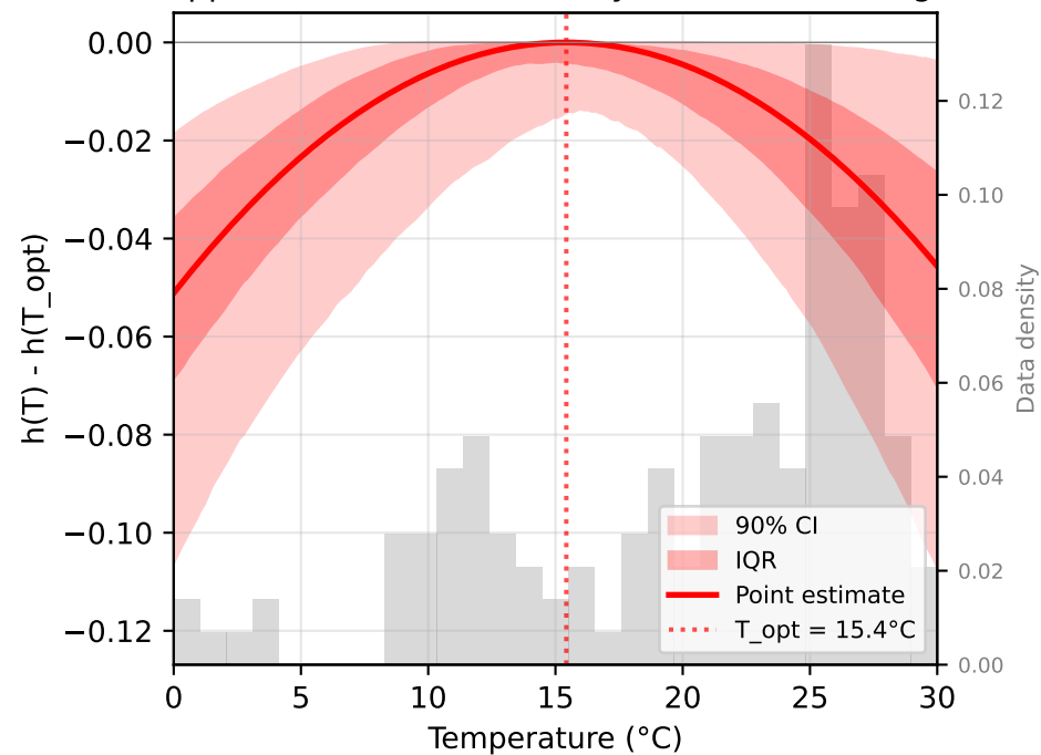
Approach1P: Quadratic (Polynomial Detrending)
