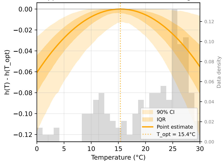
Approach1L: Quadratic (LOESS Detrending)
