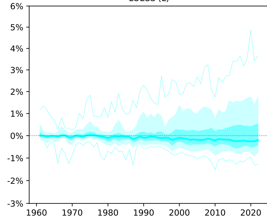
Approach DL LOESS (L)
