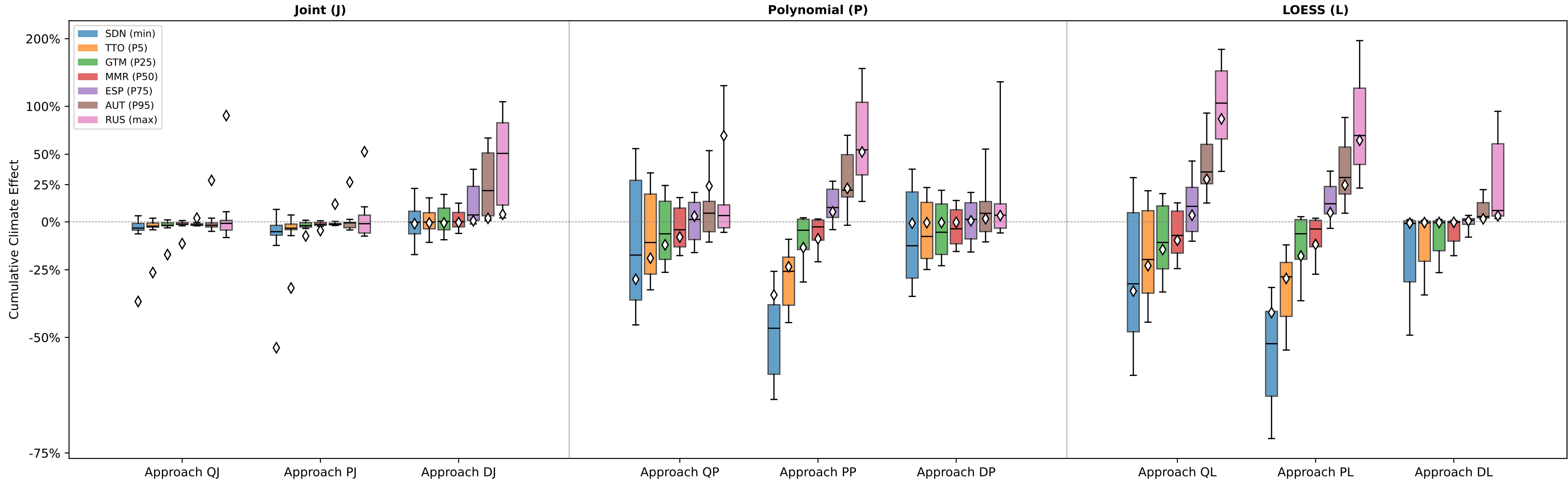
Cumulative Climate Effect on GDP Growth (1961-2022) by Approach
