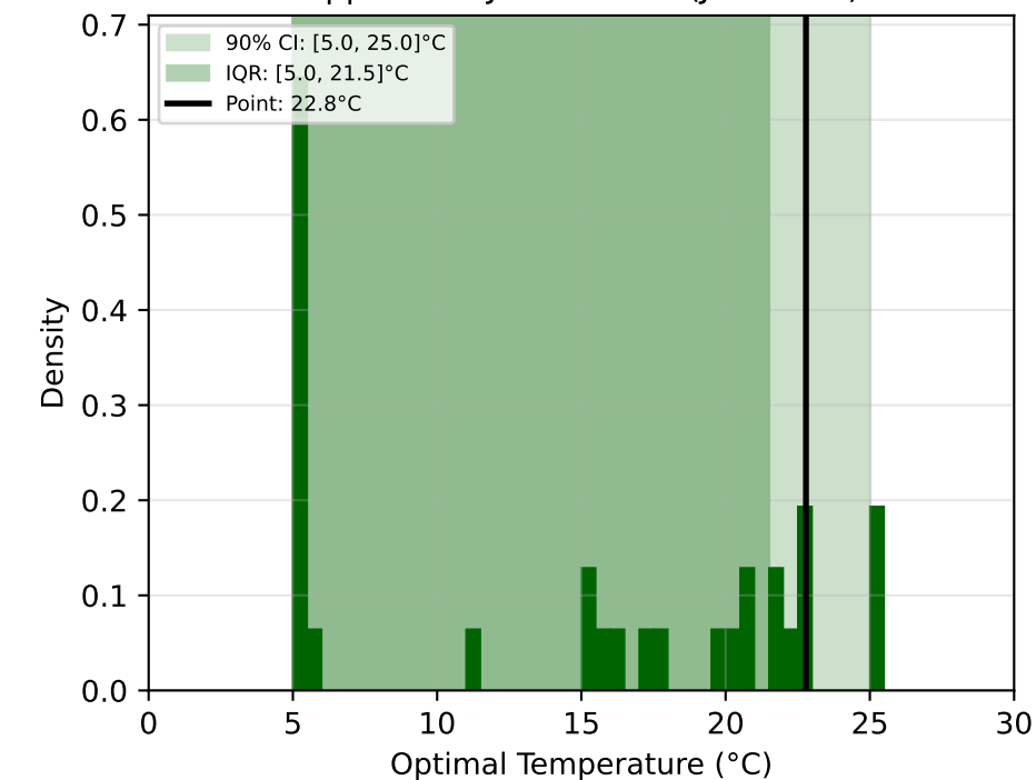
Approach DJ: Decay (Joint OLS)
