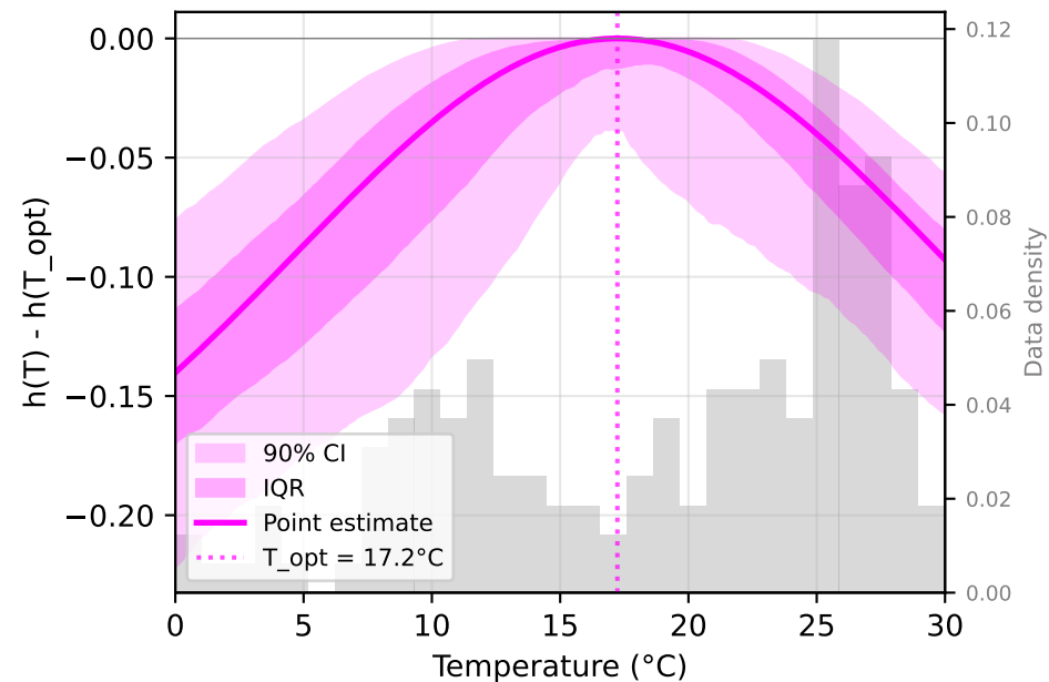
8: Gaussian LOESS
