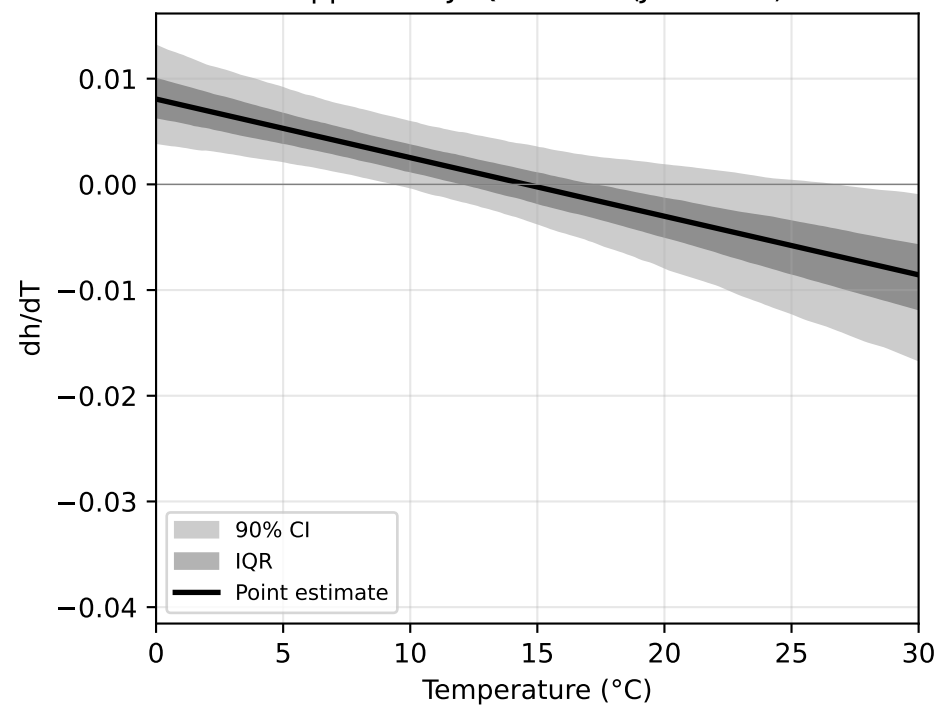
Approach1L: Quadratic (LOESS Detrending)
