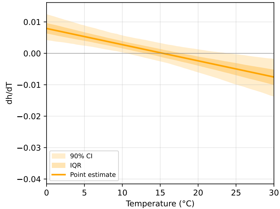
Approach3L: Persistence (LOESS Detrending)
