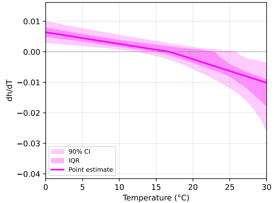
Approach2J: Piecewise (Joint OLS)
