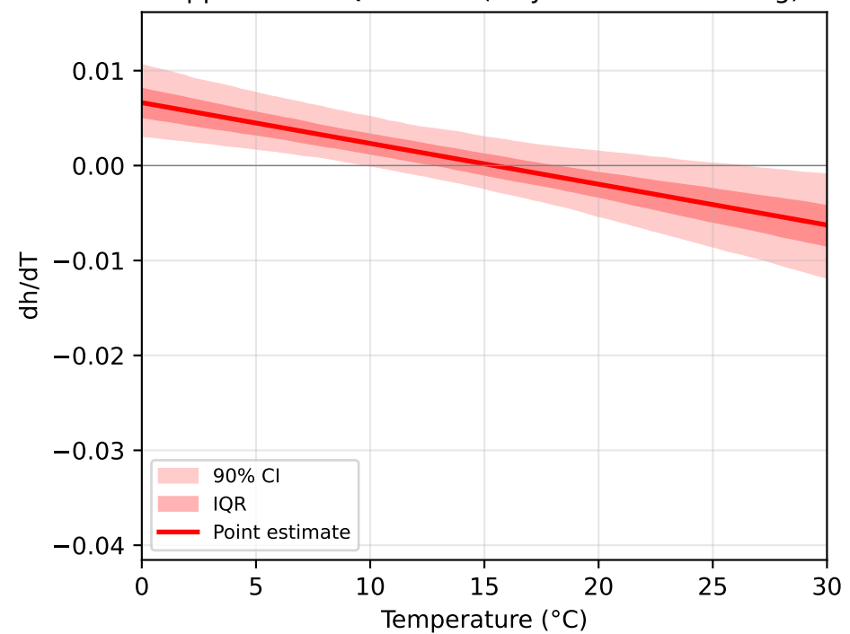
Approach2L: Piecewise (LOESS Detrending)
