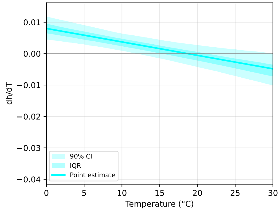
Approach3J: Persistence (Joint OLS)
