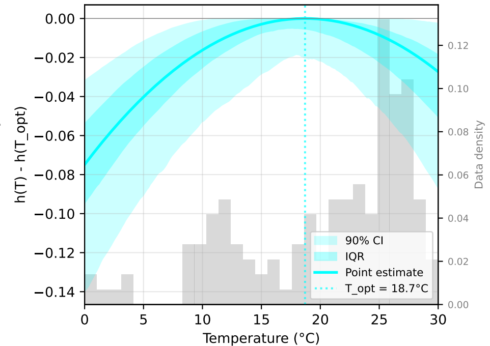
Approach3L: Persistence (LOESS Detrending)
