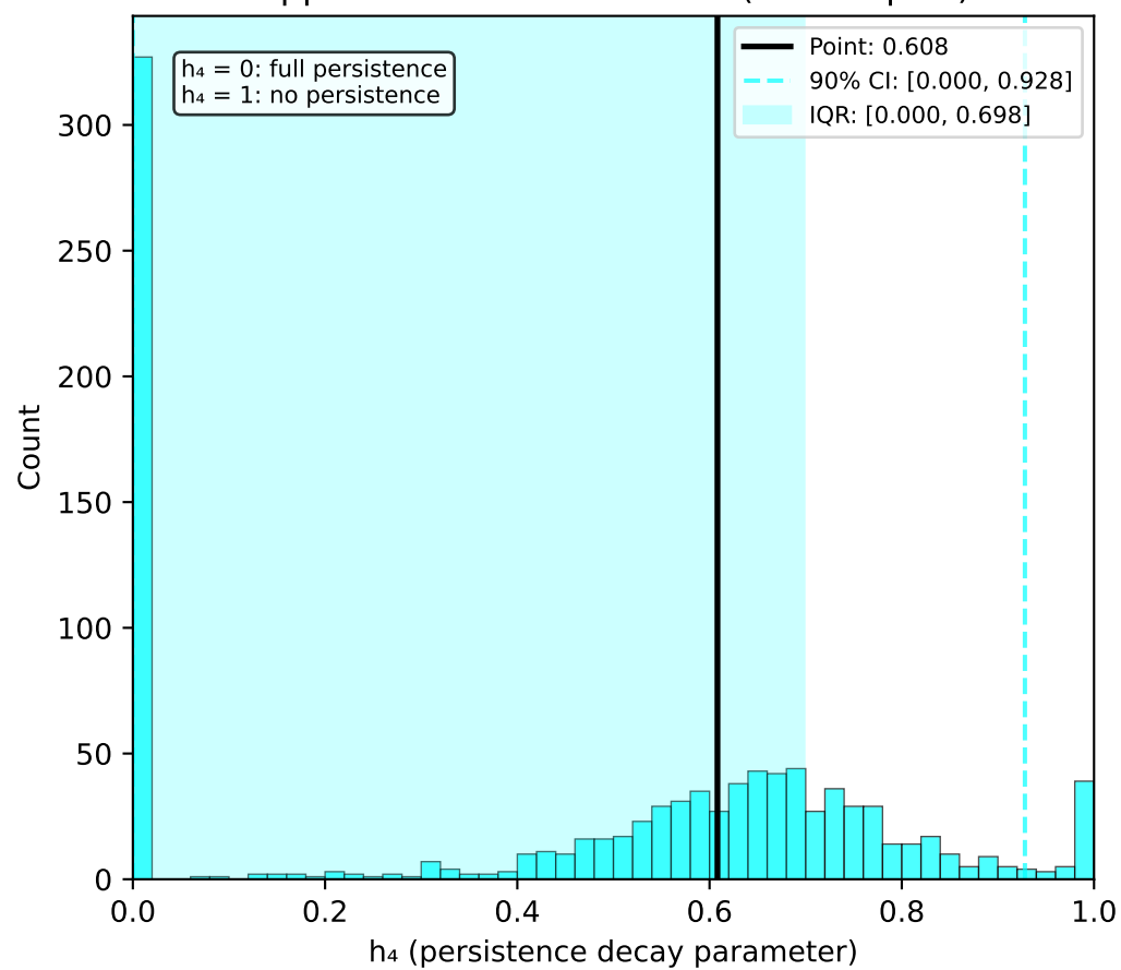
Approach 4: h_4 Distribution (All Samples)
